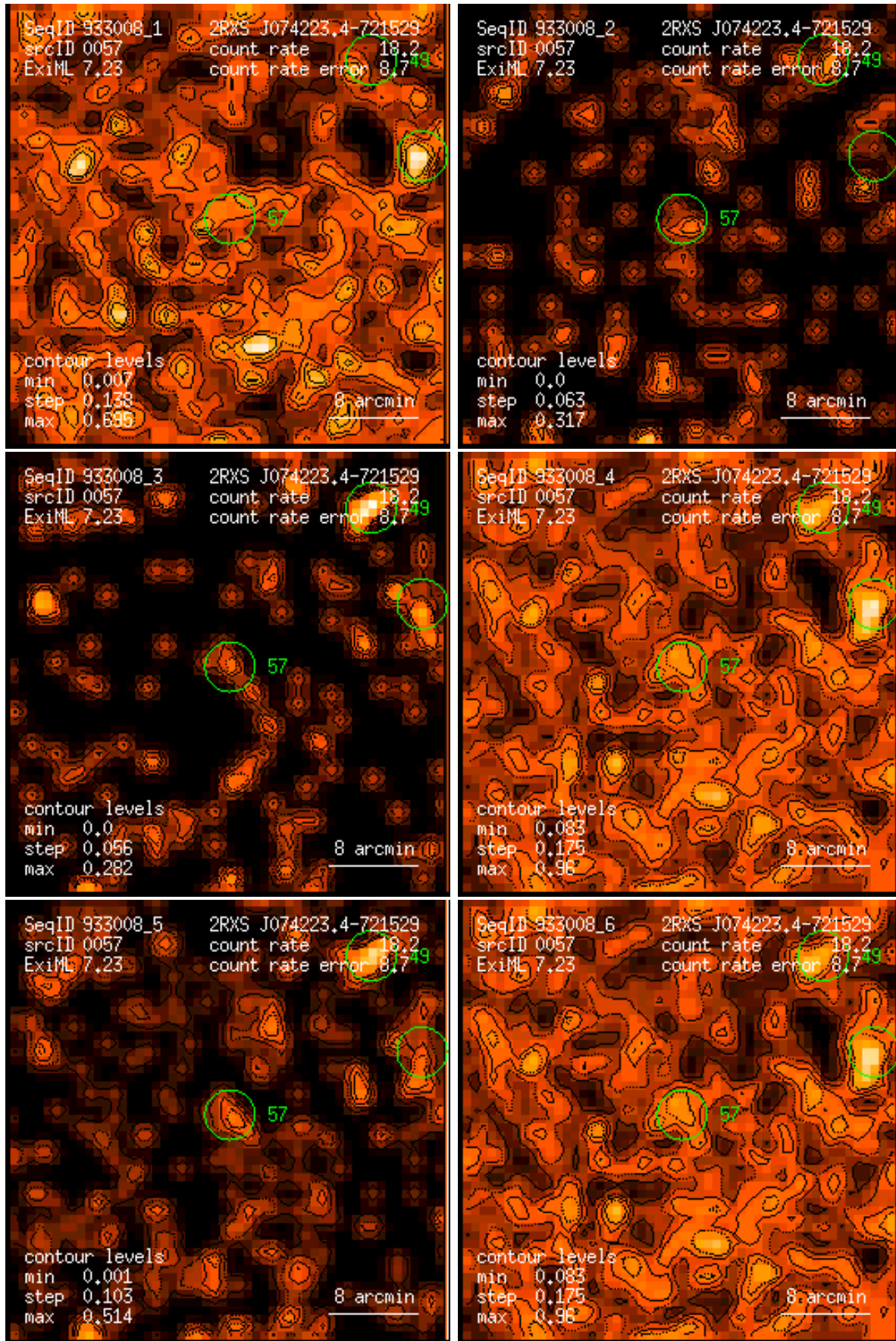
Figure 57: RASS 933008: detection 0057: band rate images, Gaussian filter: (1) PSPC channels 11 – 41, (2) 52 – 90, (3) 91 – 201, (4) 11 – 235, (5) 52 – 201, (6) 11 – 201. Broad band rates in counts/ks. Band rate contour levels in counts/ks/arcmin 2 .
