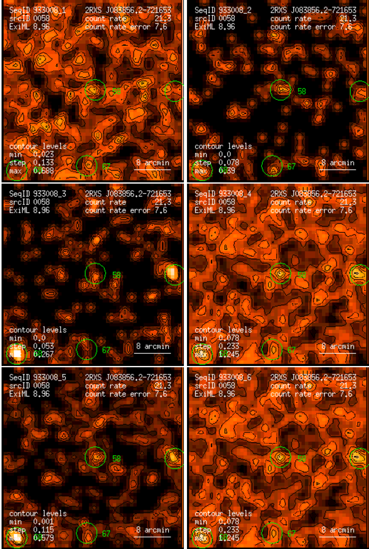
Figure 58: RASS 933008: detection 0058: band rate images, Gaussian filter: (1) PSPC channels 11 – 41, (2) 52 – 90, (3) 91 – 201, (4) 11 – 235, (5) 52 – 201, (6) 11 – 201. Broad band rates in counts/ks. Band rate contour levels in counts/ks/arcmin 2 .
