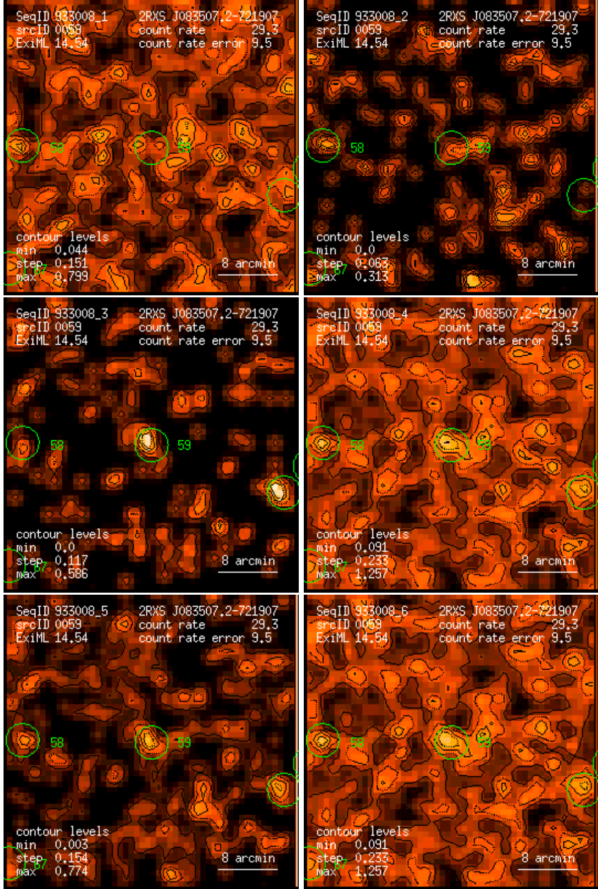
Figure 59: RASS 933008: detection 0059: band rate images, Gaussian filter: (1) PSPC channels 11 – 41, (2) 52 – 90, (3) 91 – 201, (4) 11 – 235, (5) 52 – 201, (6) 11 – 201. Broad band rates in counts/ks. Band rate contour levels in counts/ks/arcmin 2 .
