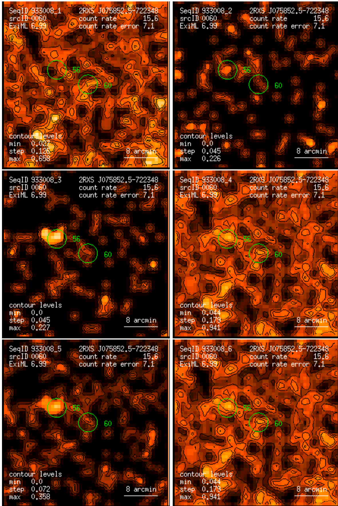
Figure 60: RASS 933008: detection 0060: band rate images, Gaussian filter: (1) PSPC channels 11 – 41, (2) 52 – 90, (3) 91 – 201, (4) 11 – 235, (5) 52 – 201, (6) 11 – 201. Broad band rates in counts/ks. Band rate contour levels in counts/ks/arcmin 2 .
