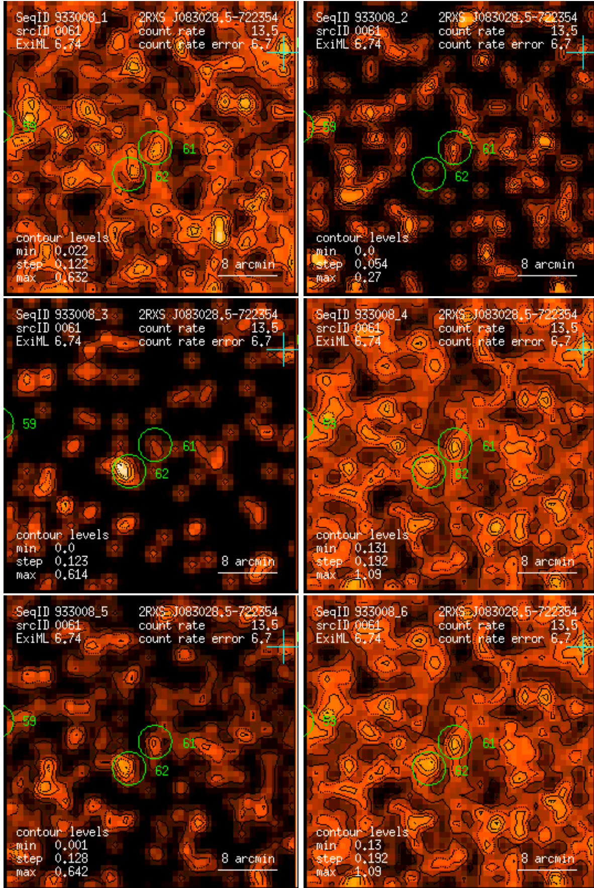
Figure 61: RASS 933008: detection 0061: band rate images, Gaussian filter: (1) PSPC channels 11 – 41, (2) 52 – 90, (3) 91 – 201, (4) 11 – 235, (5) 52 – 201, (6) 11 – 201. Broad band rates in counts/ks. Band rate contour levels in counts/ks/arcmin 2 .
