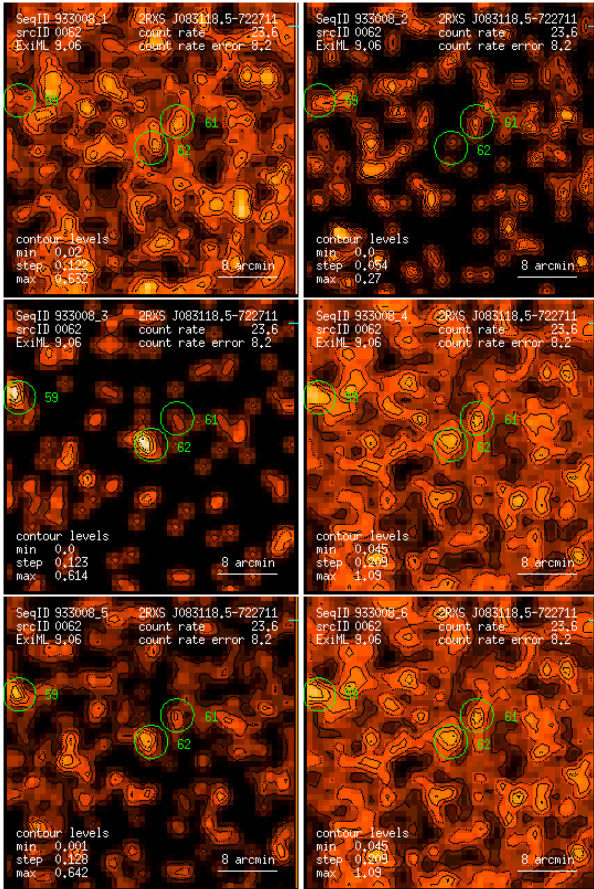
Figure 62: RASS 933008: detection 0062: band rate images, Gaussian filter: (1) PSPC channels 11 – 41, (2) 52 – 90, (3) 91 – 201, (4) 11 – 235, (5) 52 – 201, (6) 11 – 201. Broad band rates in counts/ks. Band rate contour levels in counts/ks/arcmin 2 .
