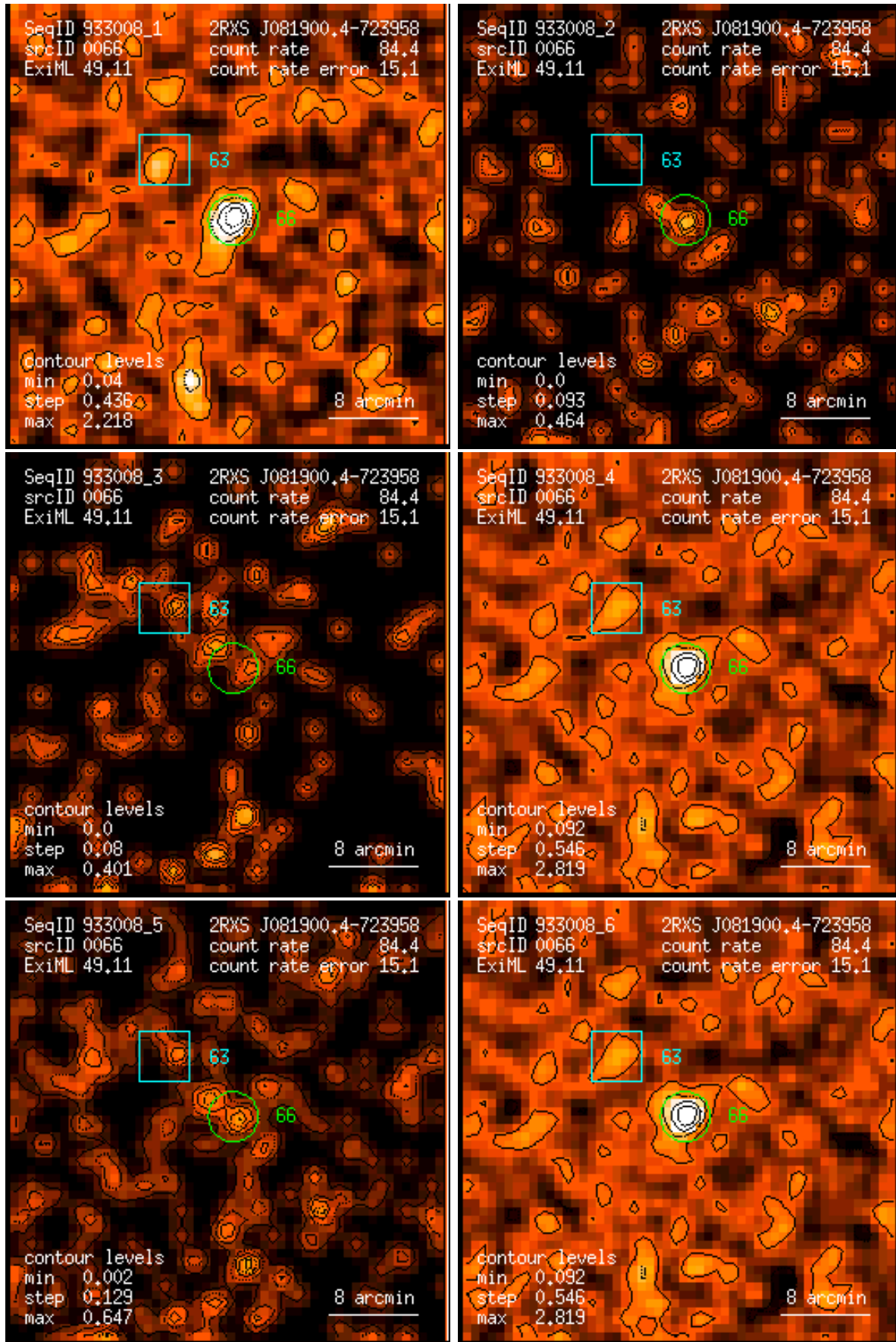
Figure 66: RASS 933008: detection 0066: band rate images, Gaussian filter: (1) PSPC channels 11 – 41, (2) 52 – 90, (3) 91 – 201, (4) 11 – 235, (5) 52 – 201, (6) 11 – 201. Broad band rates in counts/ks. Band rate contour levels in counts/ks/arcmin 2 .
