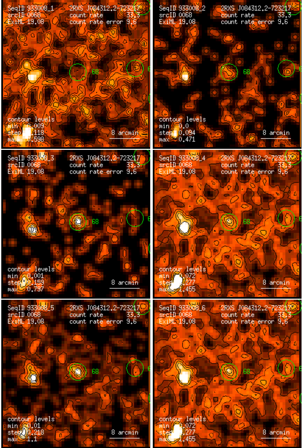
Figure 68: RASS 933008: detection 0068: band rate images, Gaussian filter: (1) PSPC channels 11 – 41, (2) 52 – 90, (3) 91 – 201, (4) 11 – 235, (5) 52 – 201, (6) 11 – 201. Broad band rates in counts/ks. Band rate contour levels in counts/ks/arcmin 2 .
