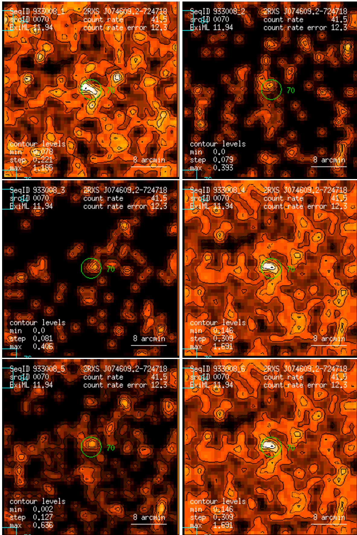
Figure 70: RASS 933008: detection 0070: band rate images, Gaussian filter: (1) PSPC channels 11 – 41, (2) 52 – 90, (3) 91 – 201, (4) 11 – 235, (5) 52 – 201, (6) 11 – 201. Broad band rates in counts/ks. Band rate contour levels in counts/ks/arcmin 2 .
