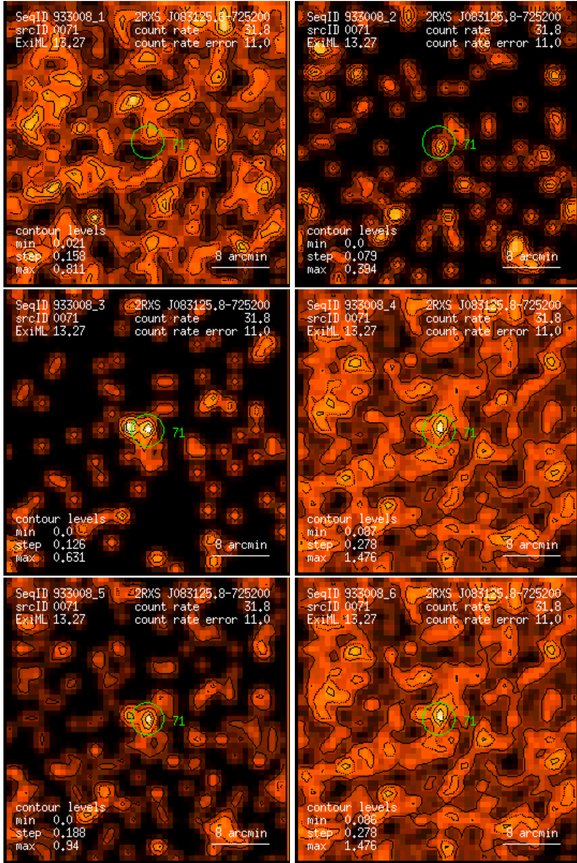
Figure 71: RASS 933008: detection 0071: band rate images, Gaussian filter: (1) PSPC channels 11 – 41, (2) 52 – 90, (3) 91 – 201, (4) 11 – 235, (5) 52 – 201, (6) 11 – 201. Broad band rates in counts/ks. Band rate contour levels in counts/ks/arcmin 2 .
