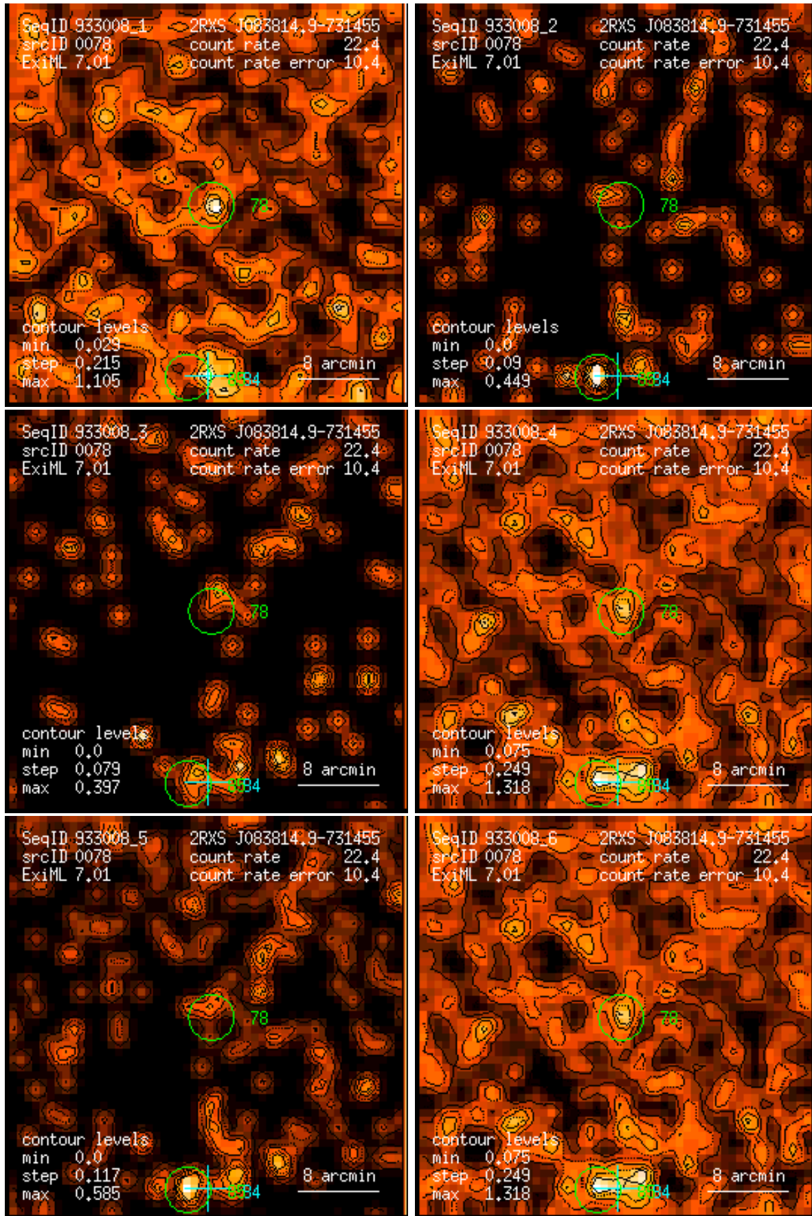
Figure 78: RASS 933008: detection 0078: band rate images, Gaussian filter: (1) PSPC channels 11 – 41, (2) 52 – 90, (3) 91 – 201, (4) 11 – 235, (5) 52 – 201, (6) 11 – 201. Broad band rates in counts/ks. Band rate contour levels in counts/ks/arcmin 2 .
