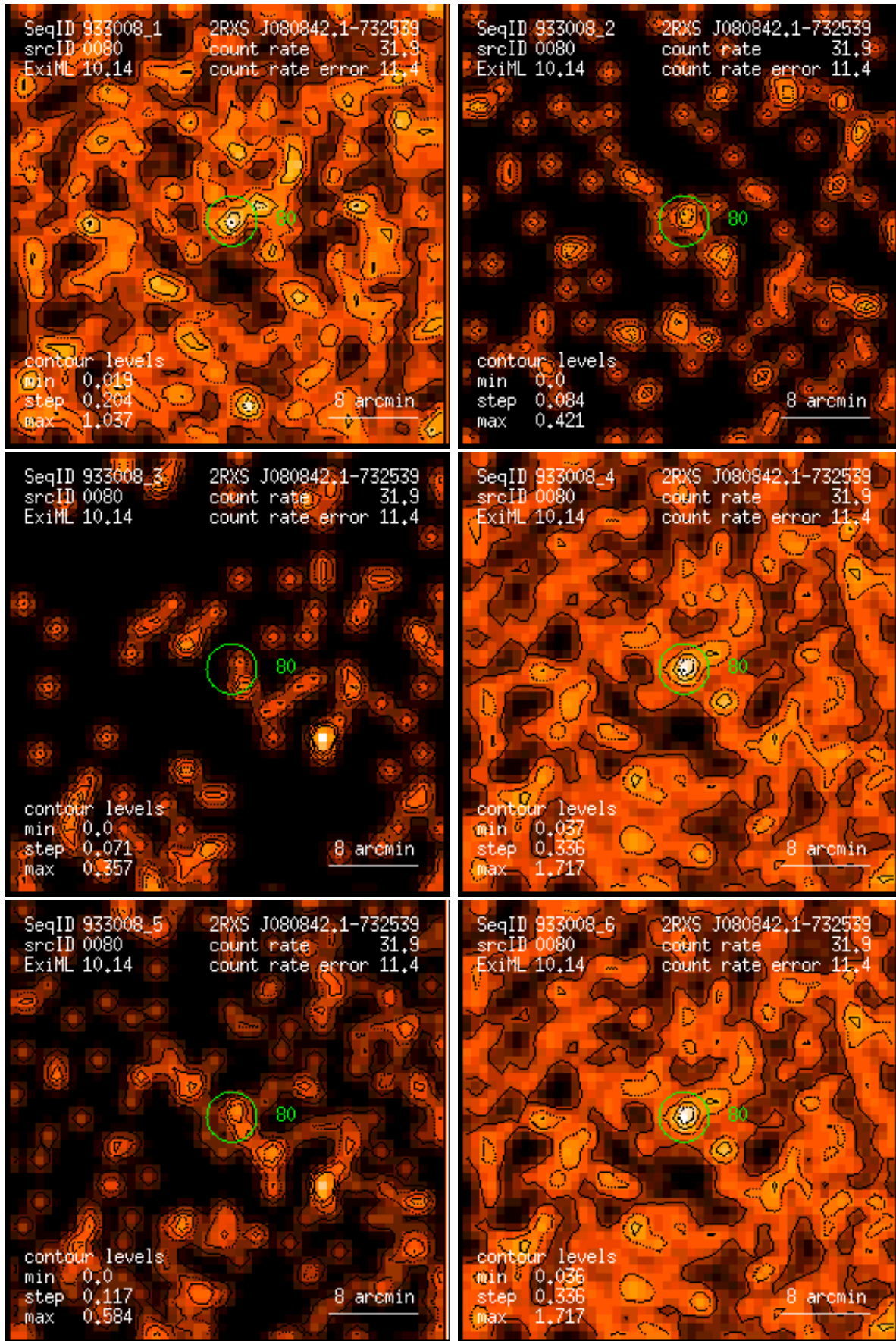
Figure 80: RASS 933008: detection 0080: band rate images, Gaussian filter: (1) PSPC channels 11 – 41, (2) 52 – 90, (3) 91 – 201, (4) 11 – 235, (5) 52 – 201, (6) 11 – 201. Broad band rates in counts/ks. Band rate contour levels in counts/ks/arcmin 2 .
