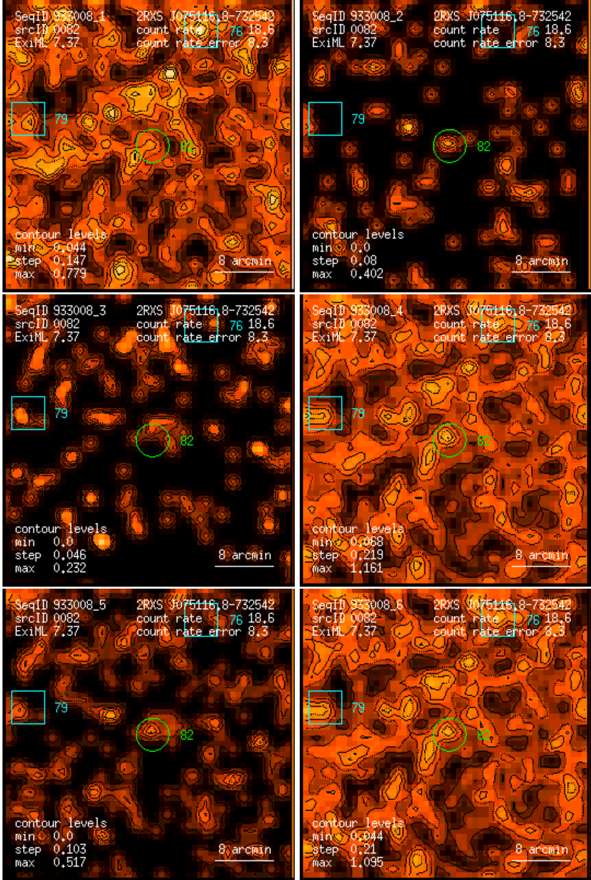
Figure 82: RASS 933008: detection 0082: band rate images, Gaussian filter: (1) PSPC channels 11 – 41, (2) 52 – 90, (3) 91 – 201, (4) 11 – 235, (5) 52 – 201, (6) 11 – 201. Broad band rates in counts/ks. Band rate contour levels in counts/ks/arcmin 2 .
