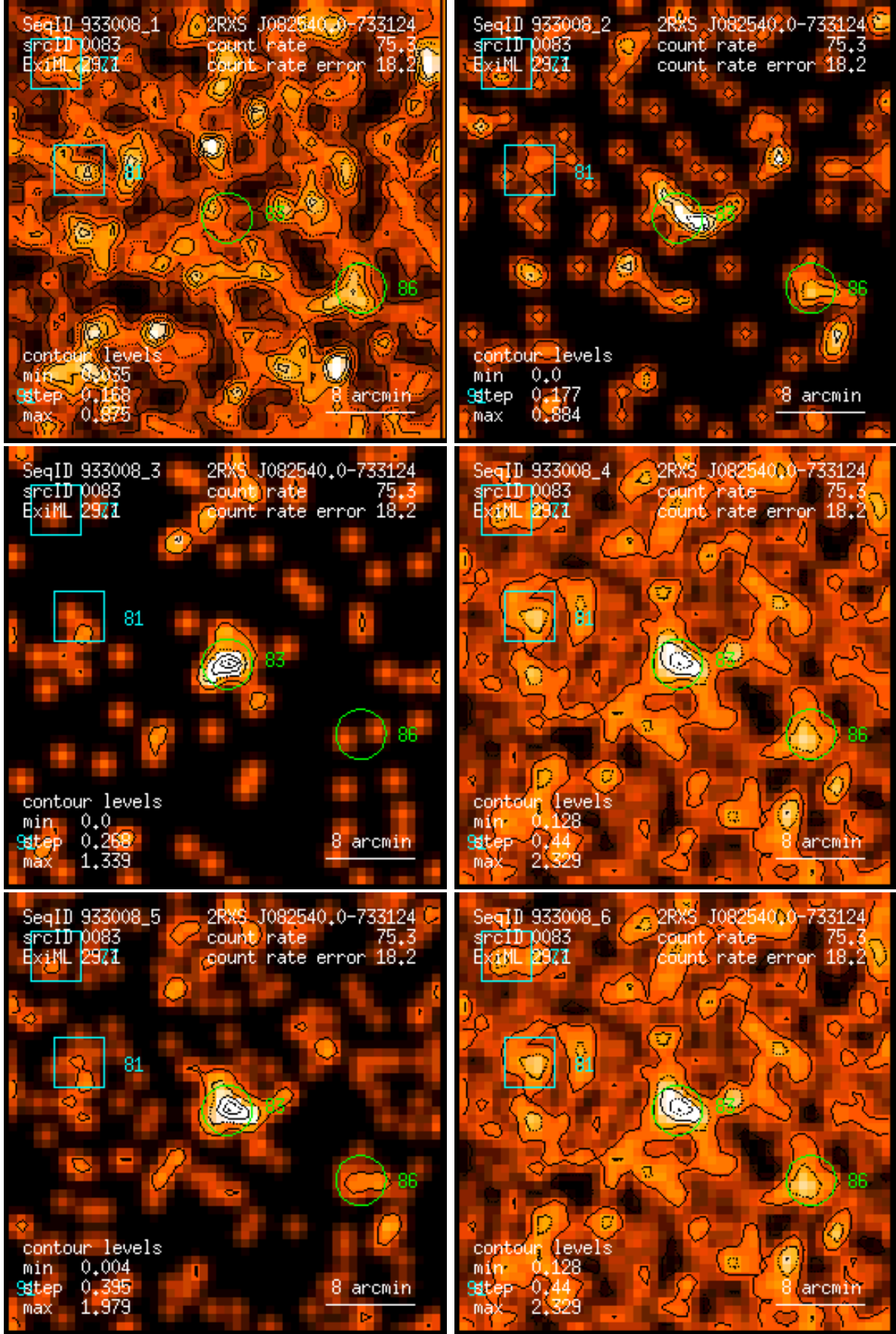
Figure 83: RASS 933008: detection 0083: band rate images, Gaussian filter: (1) PSPC channels 11 – 41, (2) 52 – 90, (3) 91 – 201, (4) 11 – 235, (5) 52 – 201, (6) 11 – 201. Broad band rates in counts/ks. Band rate contour levels in counts/ks/arcmin 2 .
