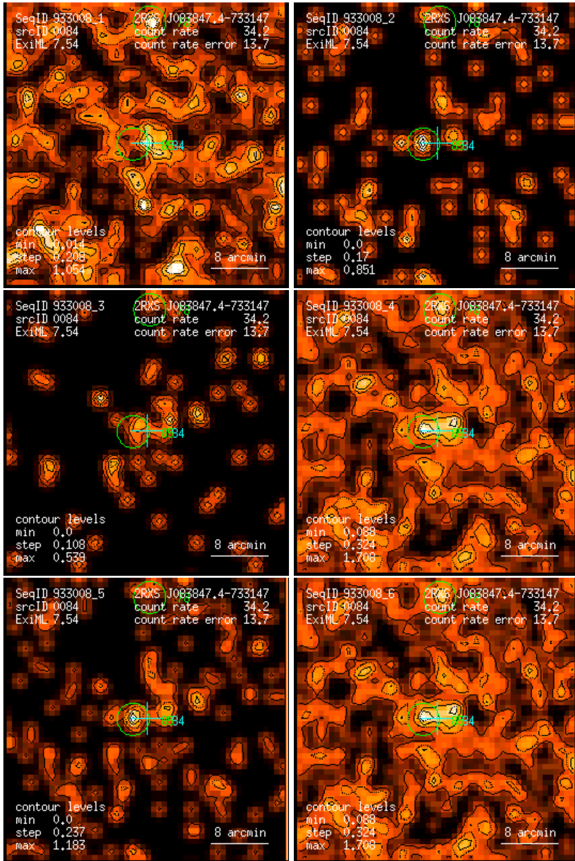
Figure 84: RASS 933008: detection 0084: band rate images, Gaussian filter: (1) PSPC channels 11 – 41, (2) 52 – 90, (3) 91 – 201, (4) 11 – 235, (5) 52 – 201, (6) 11 – 201. Broad band rates in counts/ks. Band rate contour levels in counts/ks/arcmin 2 .
