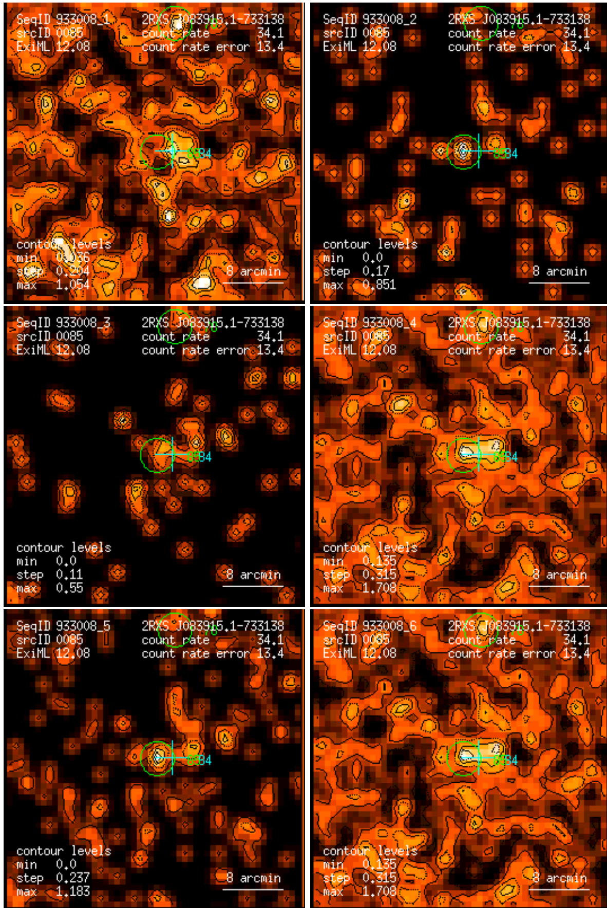
Figure 85: RASS 933008: detection 0085: band rate images, Gaussian filter: (1) PSPC channels 11 – 41, (2) 52 – 90, (3) 91 – 201, (4) 11 – 235, (5) 52 – 201, (6) 11 – 201. Broad band rates in counts/ks. Band rate contour levels in counts/ks/arcmin 2 .
