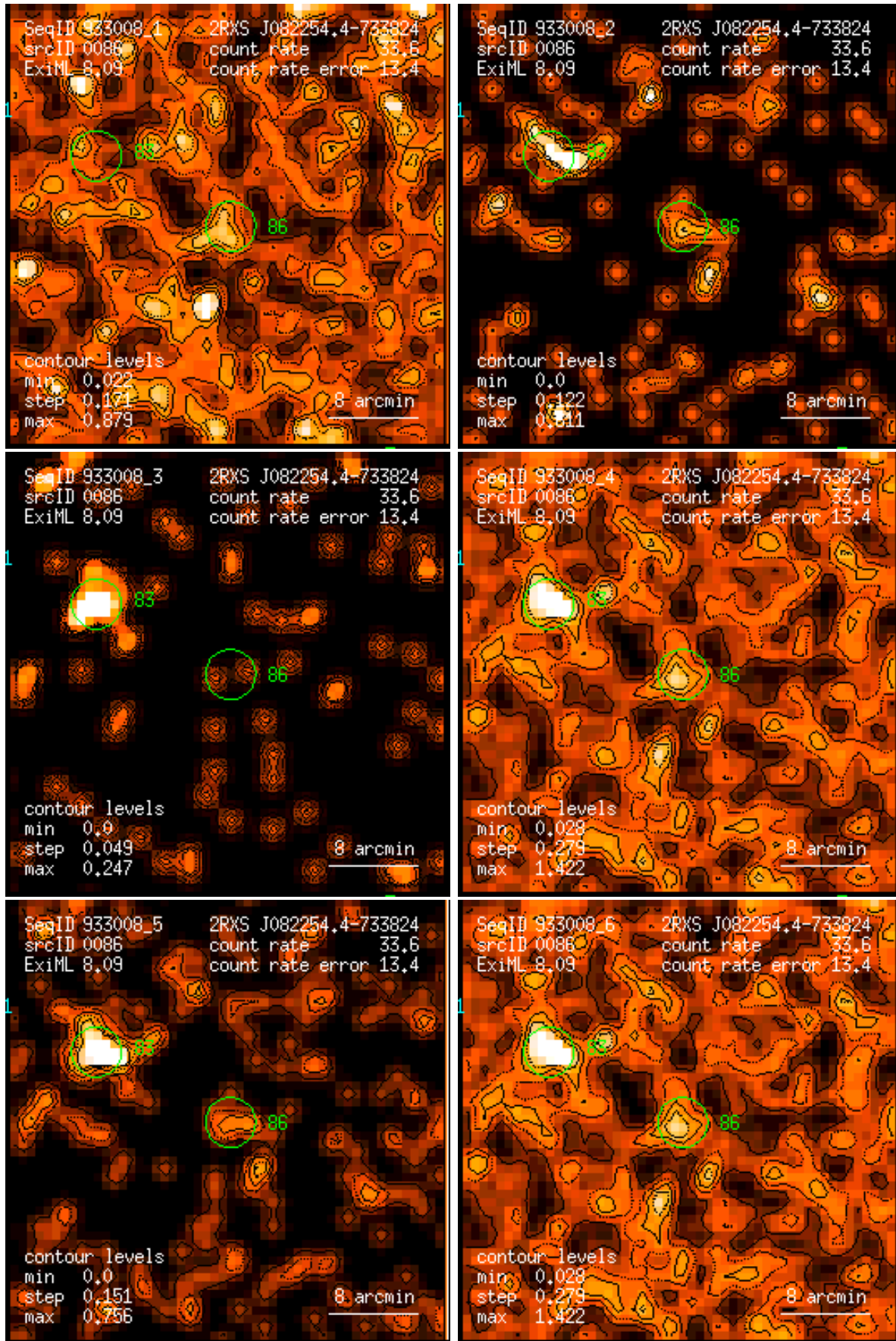
Figure 86: RASS 933008: detection 0086: band rate images, Gaussian filter: (1) PSPC channels 11 – 41, (2) 52 – 90, (3) 91 – 201, (4) 11 – 235, (5) 52 – 201, (6) 11 – 201. Broad band rates in counts/ks. Band rate contour levels in counts/ks/arcmin 2 .
