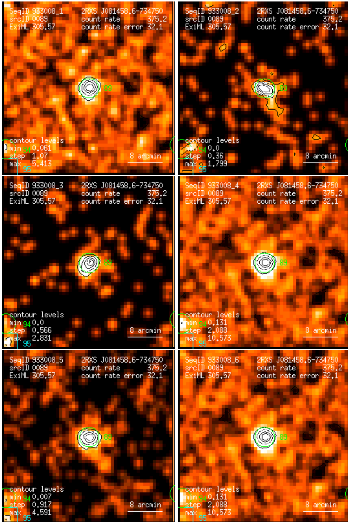
Figure 89: RASS 933008: detection 0089: band rate images, Gaussian filter: (1) PSPC channels 11 – 41, (2) 52 – 90, (3) 91 – 201, (4) 11 – 235, (5) 52 – 201, (6) 11 – 201. Broad band rates in counts/ks. Band rate contour levels in counts/ks/arcmin 2 .
