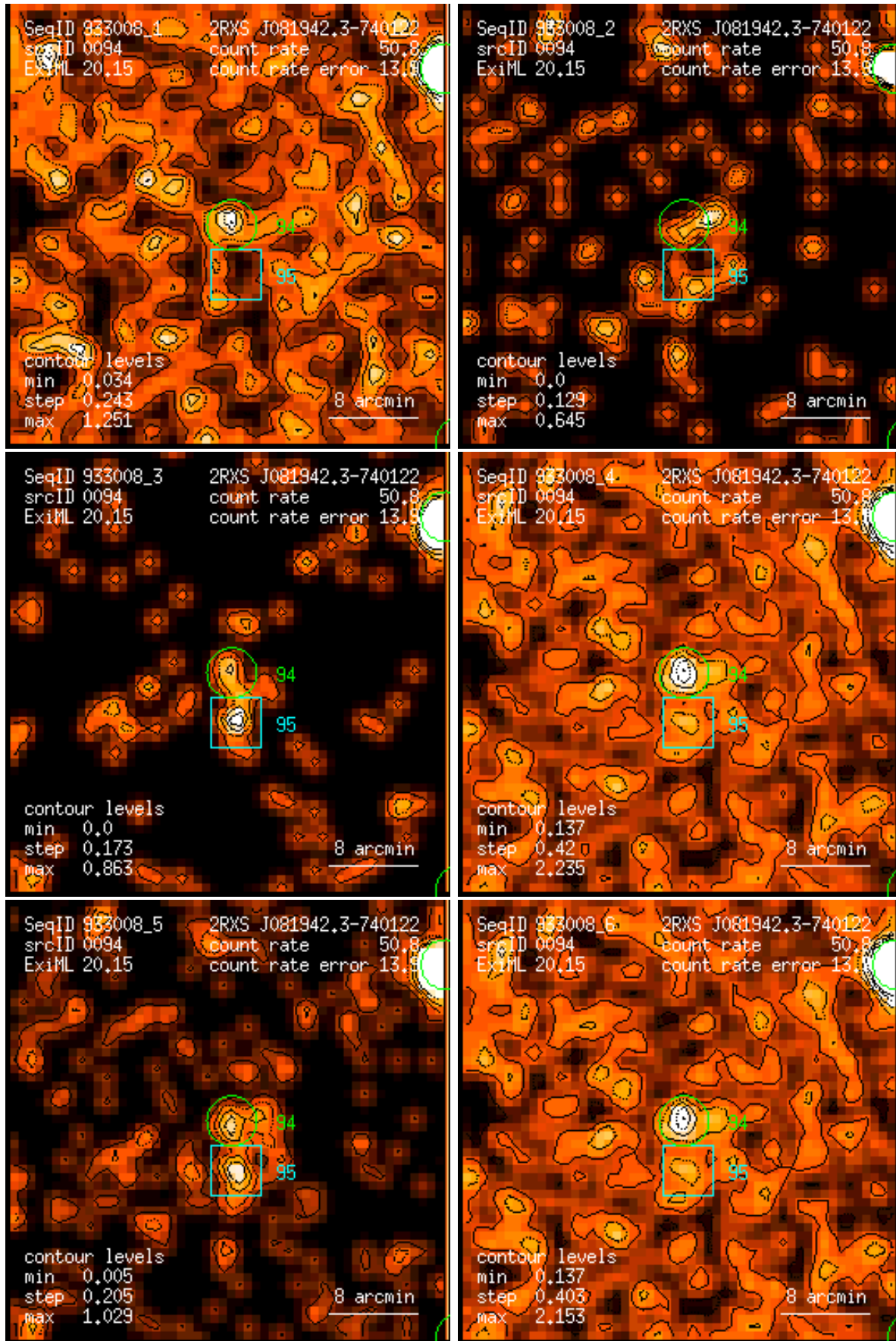
Figure 94: RASS 933008: detection 0094: band rate images, Gaussian filter: (1) PSPC channels 11 – 41, (2) 52 – 90, (3) 91 – 201, (4) 11 – 235, (5) 52 – 201, (6) 11 – 201. Broad band rates in counts/ks. Band rate contour levels in counts/ks/arcmin 2 .
