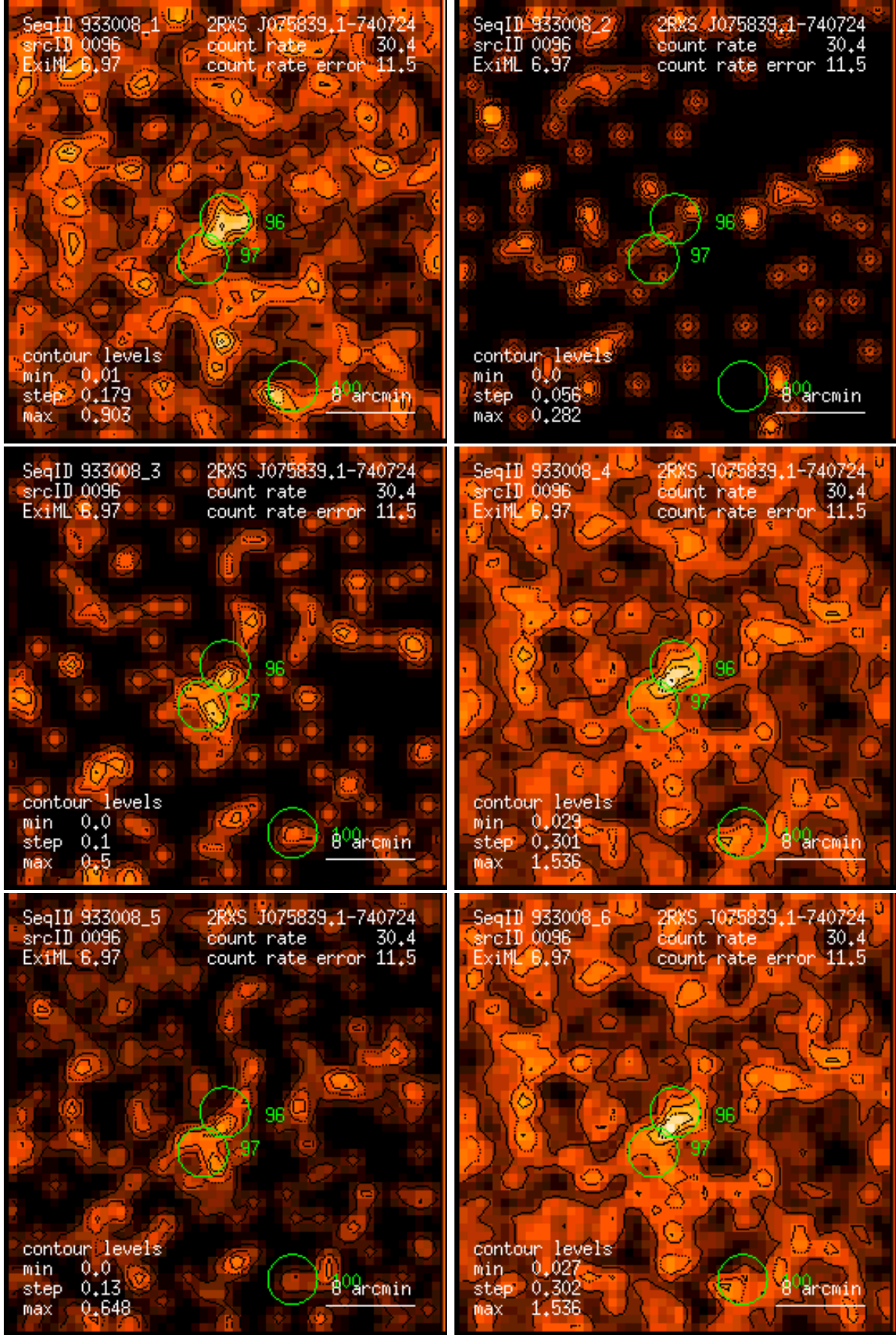
Figure 96: RASS 933008: detection 0096: band rate images, Gaussian filter: (1) PSPC channels 11 – 41, (2) 52 – 90, (3) 91 – 201, (4) 11 – 235, (5) 52 – 201, (6) 11 – 201. Broad band rates in counts/ks. Band rate contour levels in counts/ks/arcmin 2 .
