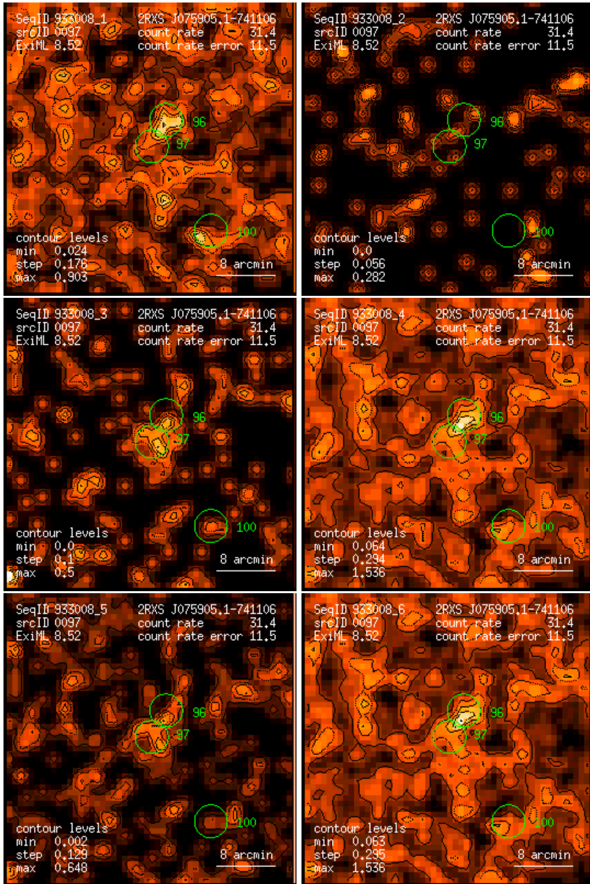
Figure 97: RASS 933008: detection 0097: band rate images, Gaussian filter: (1) PSPC channels 11 – 41, (2) 52 – 90, (3) 91 – 201, (4) 11 – 235, (5) 52 – 201, (6) 11 – 201. Broad band rates in counts/ks. Band rate contour levels in counts/ks/arcmin 2 .
