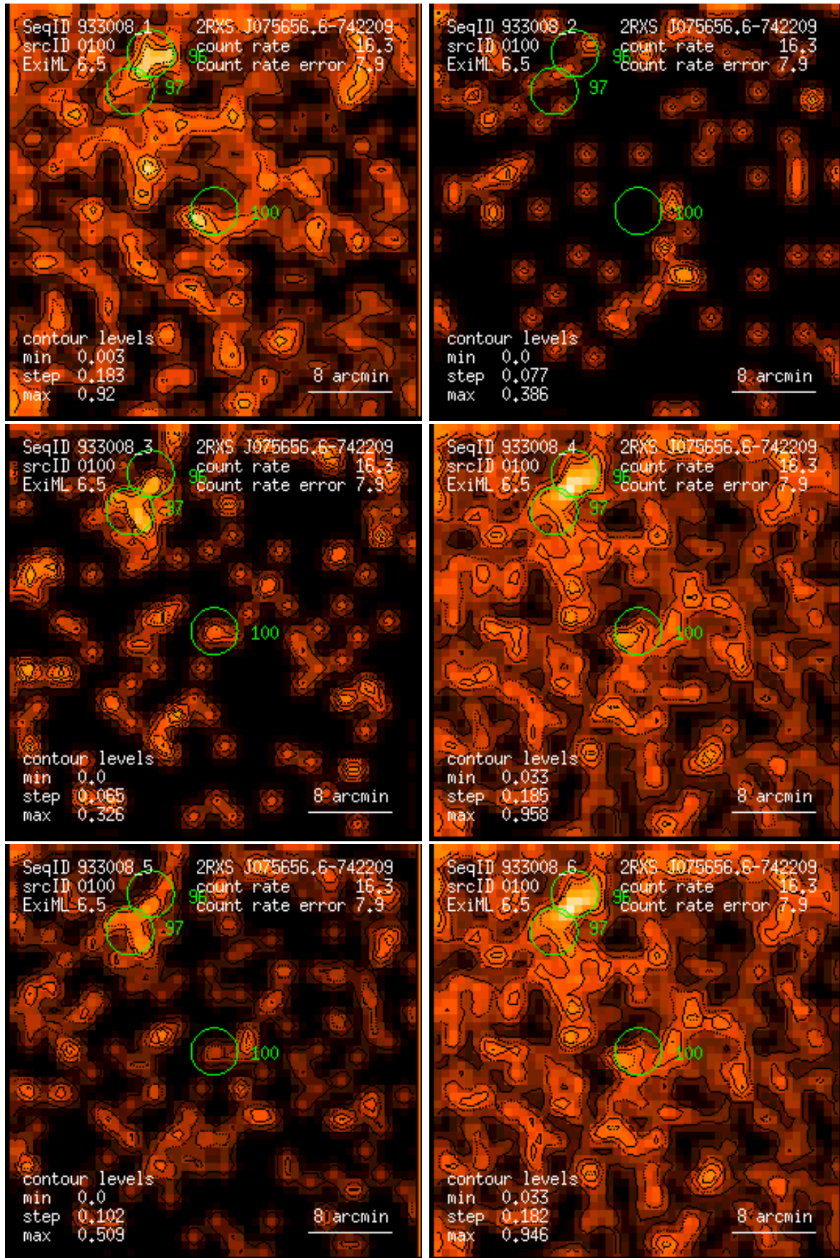
Figure 100: RASS 933008: detection 0100: band rate images, Gaussian filter: (1) PSPC channels 11 – 41, (2) 52 – 90, (3) 91 – 201, (4) 11 – 235, (5) 52 – 201, (6) 11 – 201. Broad band rates in counts/ks. Band rate contour levels in counts/ks/arcmin 2 .
