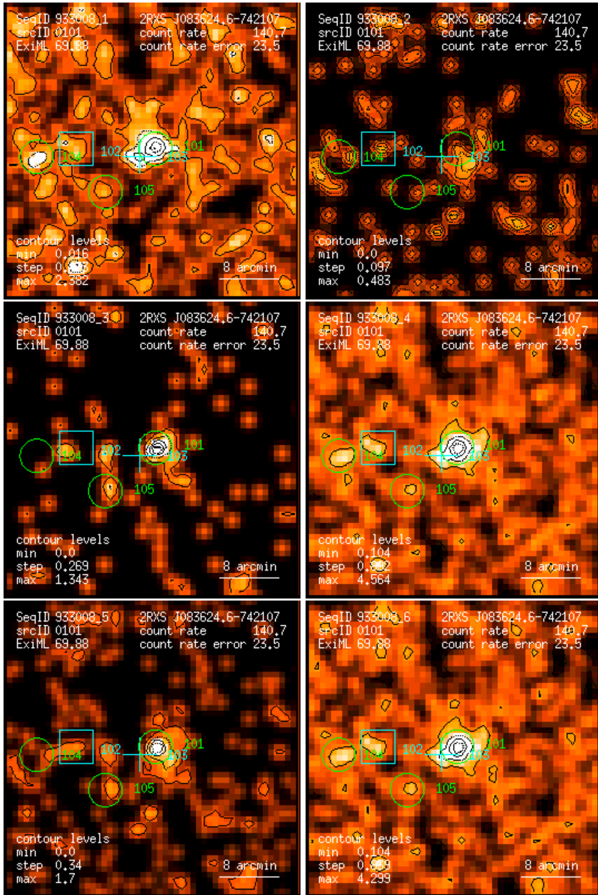
Figure 101: RASS 933008: detection 0101: band rate images, Gaussian filter: (1) PSPC channels 11 – 41, (2) 52 – 90, (3) 91 – 201, (4) 11 – 235, (5) 52 – 201, (6) 11 – 201. Broad band rates in counts/ks. Band rate contour levels in counts/ks/arcmin 2 .
