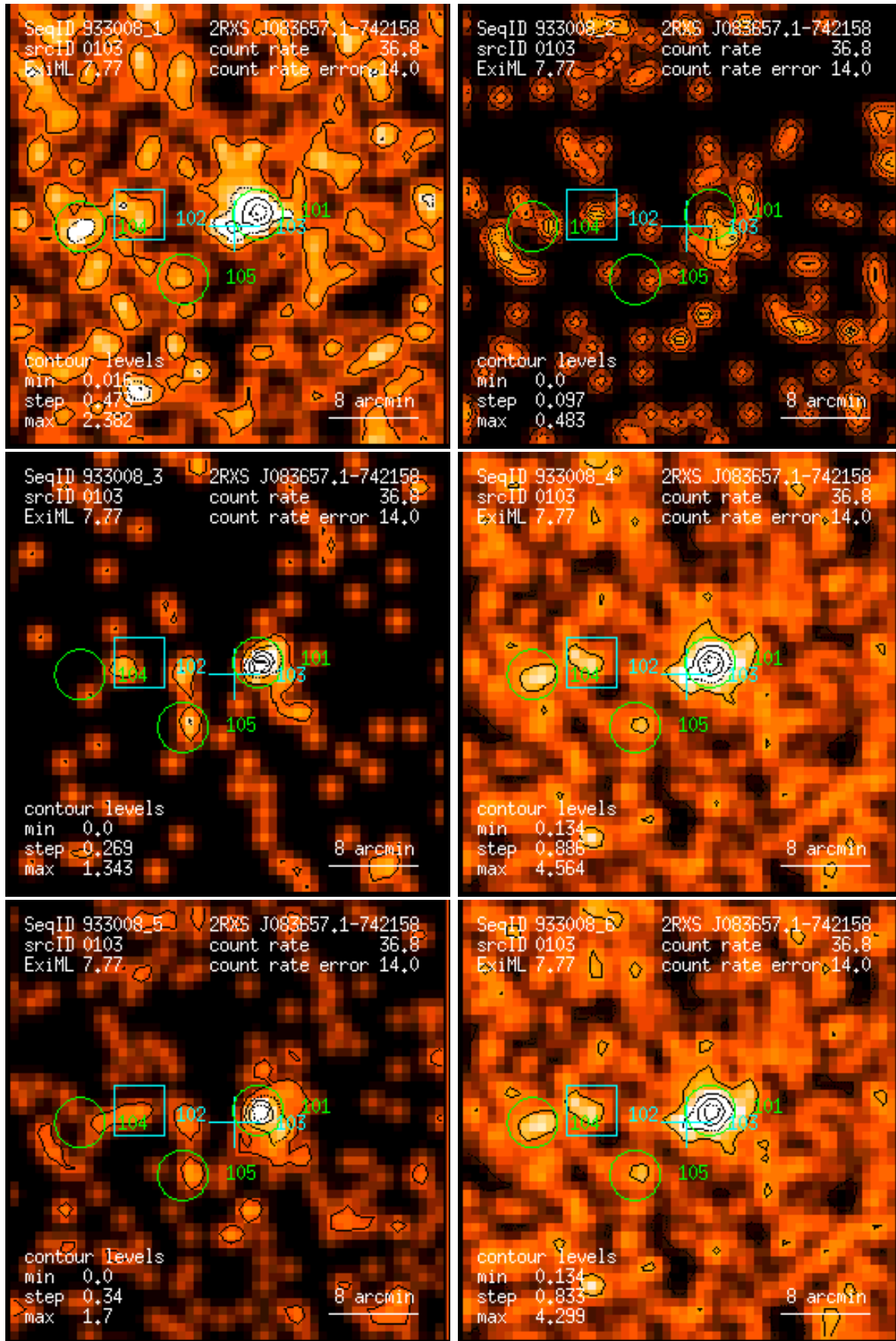
Figure 103: RASS 933008: detection 0103: band rate images, Gaussian filter: (1) PSPC channels 11 – 41, (2) 52 – 90, (3) 91 – 201, (4) 11 – 235, (5) 52 – 201, (6) 11 – 201. Broad band rates in counts/ks. Band rate contour levels in counts/ks/arcmin 2 .
