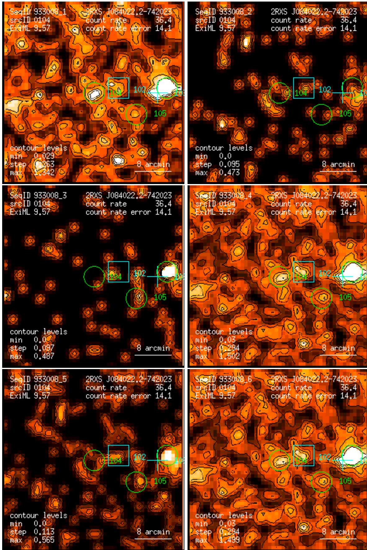
Figure 104: RASS 933008: detection 0104: band rate images, Gaussian filter: (1) PSPC channels 11 – 41, (2) 52 – 90, (3) 91 – 201, (4) 11 – 235, (5) 52 – 201, (6) 11 – 201. Broad band rates in counts/ks. Band rate contour levels in counts/ks/arcmin 2 .
