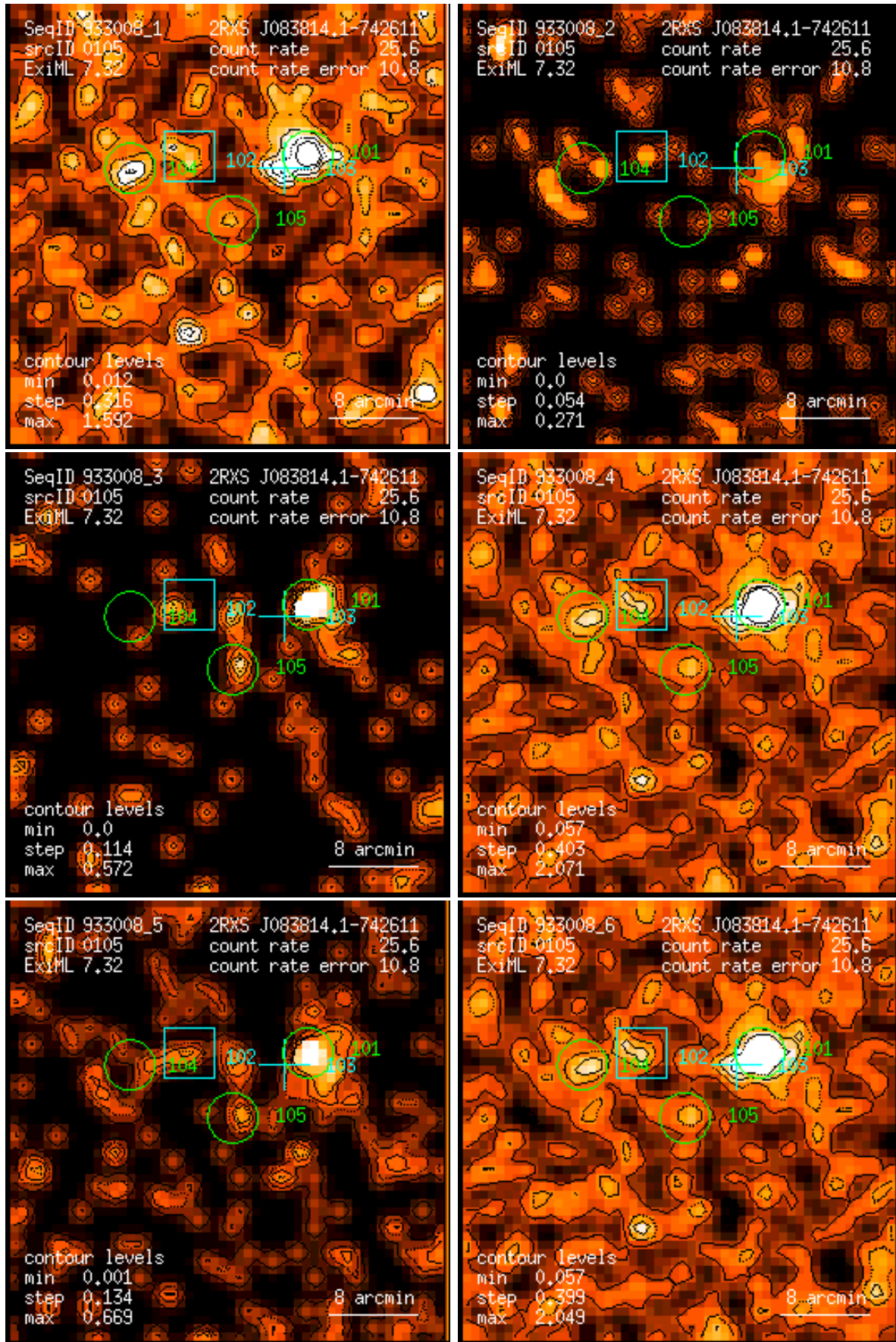
Figure 105: RASS 933008: detection 0105: band rate images, Gaussian filter: (1) PSPC channels 11 – 41, (2) 52 – 90, (3) 91 – 201, (4) 11 – 235, (5) 52 – 201, (6) 11 – 201. Broad band rates in counts/ks. Band rate contour levels in counts/ks/arcmin 2 .
