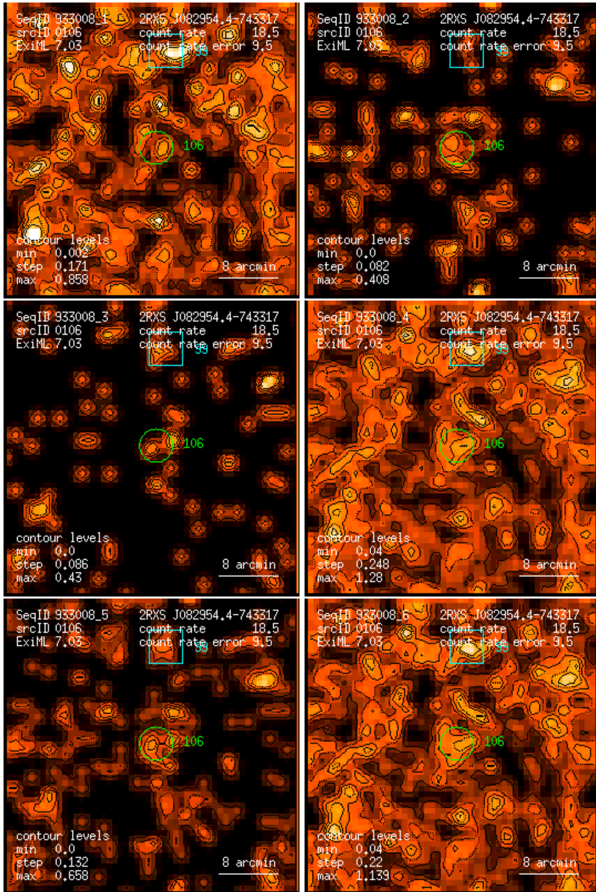
Figure 106: RASS 933008: detection 0106: band rate images, Gaussian filter: (1) PSPC channels 11 – 41, (2) 52 – 90, (3) 91 – 201, (4) 11 – 235, (5) 52 – 201, (6) 11 – 201. Broad band rates in counts/ks. Band rate contour levels in counts/ks/arcmin 2 .
