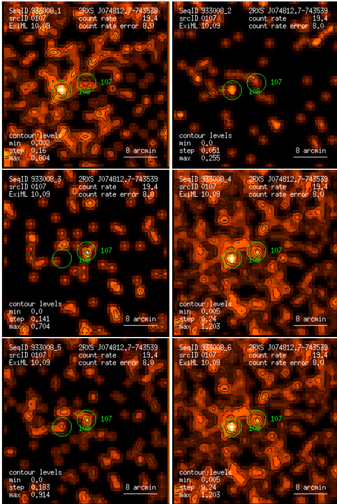
Figure 107: RASS 933008: detection 0107: band rate images, Gaussian filter: (1) PSPC channels 11 – 41, (2) 52 – 90, (3) 91 – 201, (4) 11 – 235, (5) 52 – 201, (6) 11 – 201. Broad band rates in counts/ks. Band rate contour levels in counts/ks/arcmin 2 .
