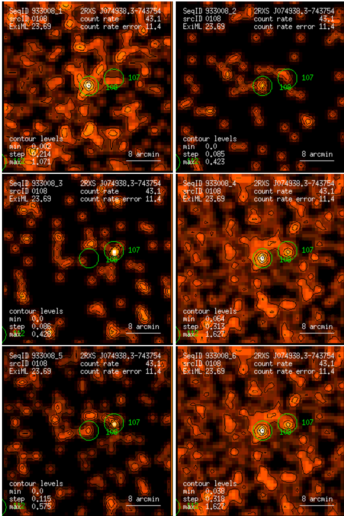
Figure 108: RASS 933008: detection 0108: band rate images, Gaussian filter: (1) PSPC channels 11 – 41, (2) 52 – 90, (3) 91 – 201, (4) 11 – 235, (5) 52 – 201, (6) 11 – 201. Broad band rates in counts/ks. Band rate contour levels in counts/ks/arcmin 2 .
