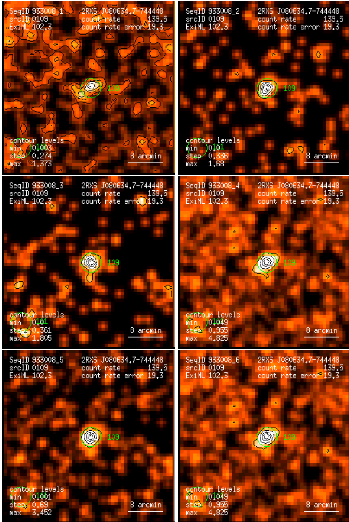
Figure 109: RASS 933008: detection 0109: band rate images, Gaussian filter: (1) PSPC channels 11 – 41, (2) 52 – 90, (3) 91 – 201, (4) 11 – 235, (5) 52 – 201, (6) 11 – 201. Broad band rates in counts/ks. Band rate contour levels in counts/ks/arcmin 2 .
