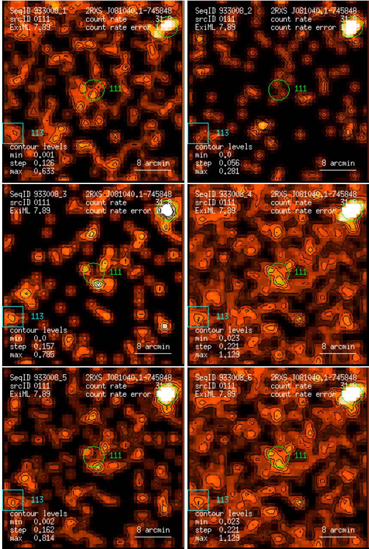
Figure 111: RASS 933008: detection 0111: band rate images, Gaussian filter: (1) PSPC channels 11 – 41, (2) 52 – 90, (3) 91 – 201, (4) 11 – 235, (5) 52 – 201, (6) 11 – 201. Broad band rates in counts/ks. Band rate contour levels in counts/ks/arcmin 2 .
