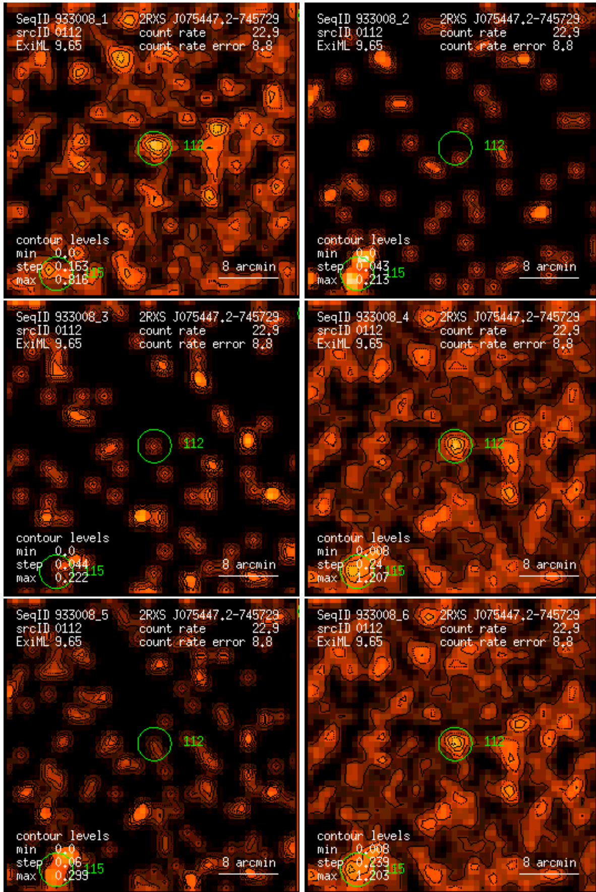
Figure 112: RASS 933008: detection 0112: band rate images, Gaussian filter: (1) PSPC channels 11 – 41, (2) 52 – 90, (3) 91 – 201, (4) 11 – 235, (5) 52 – 201, (6) 11 – 201. Broad band rates in counts/ks. Band rate contour levels in counts/ks/arcmin 2 .
