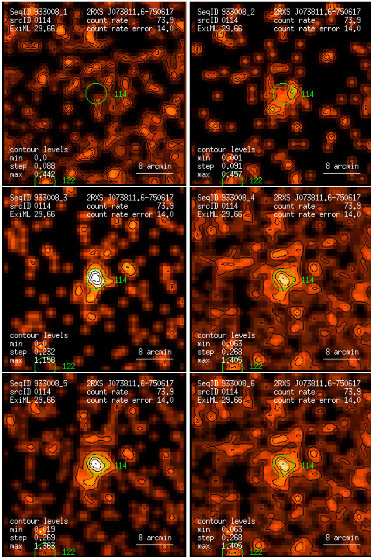
Figure 114: RASS 933008: detection 0114: band rate images, Gaussian filter: (1) PSPC channels 11 – 41, (2) 52 – 90, (3) 91 – 201, (4) 11 – 235, (5) 52 – 201, (6) 11 – 201. Broad band rates in counts/ks. Band rate contour levels in counts/ks/arcmin 2 .
