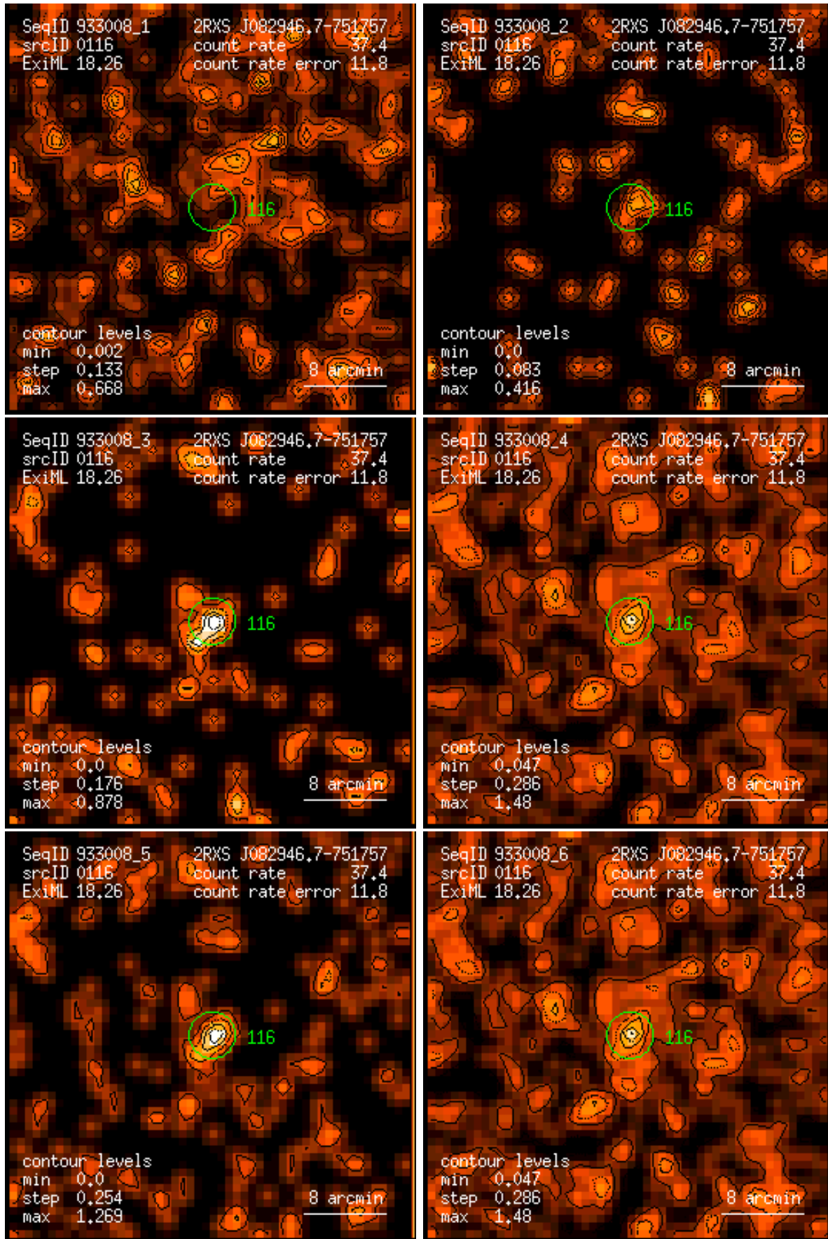
Figure 116: RASS 933008: detection 0116: band rate images, Gaussian filter: (1) PSPC channels 11 – 41, (2) 52 – 90, (3) 91 – 201, (4) 11 – 235, (5) 52 – 201, (6) 11 – 201. Broad band rates in counts/ks. Band rate contour levels in counts/ks/arcmin 2 .
