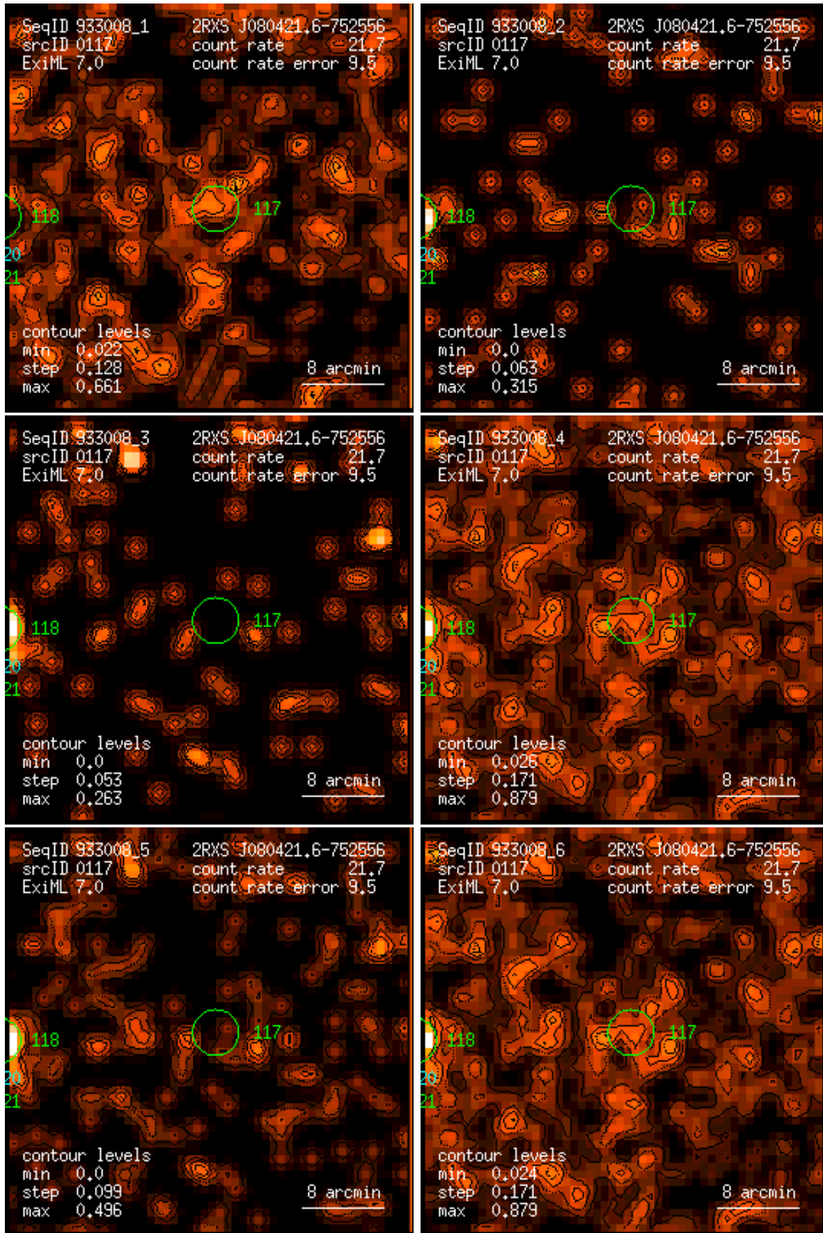
Figure 117: RASS 933008: detection 0117: band rate images, Gaussian filter: (1) PSPC channels 11 – 41, (2) 52 – 90, (3) 91 – 201, (4) 11 – 235, (5) 52 – 201, (6) 11 – 201. Broad band rates in counts/ks. Band rate contour levels in counts/ks/arcmin 2 .
