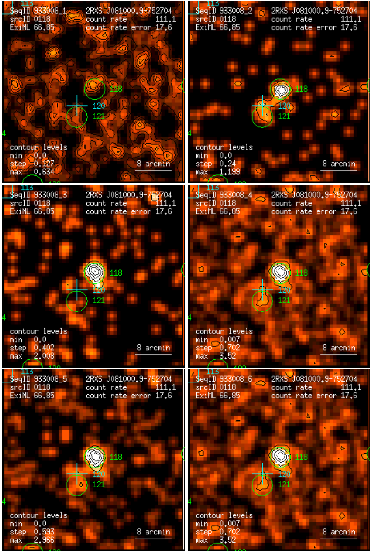
Figure 118: RASS 933008: detection 0118: band rate images, Gaussian filter: (1) PSPC channels 11 – 41, (2) 52 – 90, (3) 91 – 201, (4) 11 – 235, (5) 52 – 201, (6) 11 – 201. Broad band rates in counts/ks. Band rate contour levels in counts/ks/arcmin 2 .
