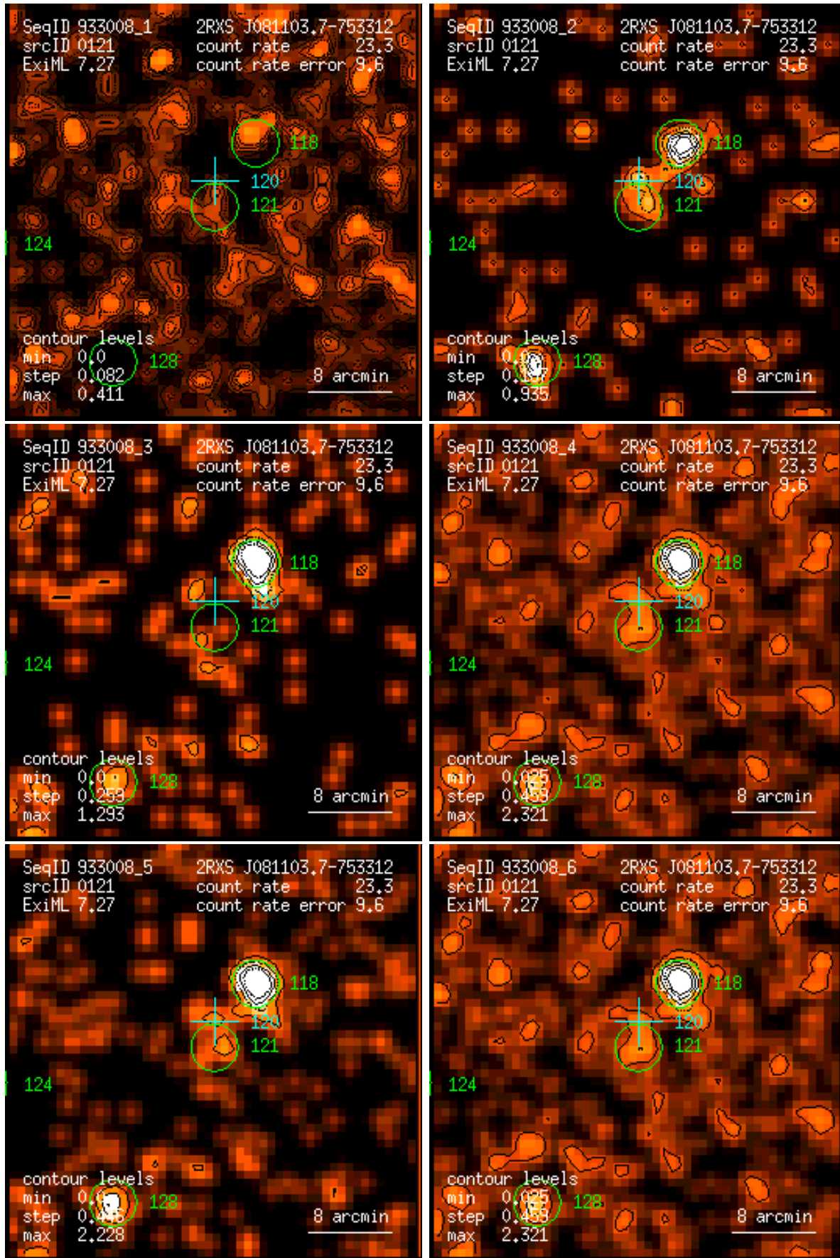
Figure 121: RASS 933008: detection 0121: band rate images, Gaussian filter: (1) PSPC channels 11 – 41, (2) 52 – 90, (3) 91 – 201, (4) 11 – 235, (5) 52 – 201, (6) 11 – 201. Broad band rates in counts/ks. Band rate contour levels in counts/ks/arcmin 2 .
