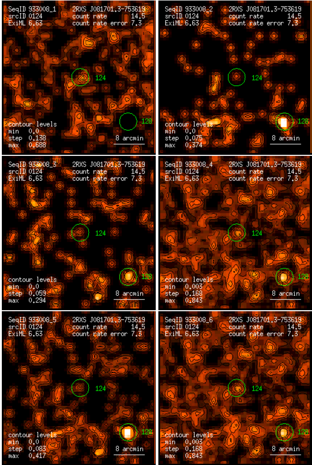
Figure 124: RASS 933008: detection 0124: band rate images, Gaussian filter: (1) PSPC channels 11 – 41, (2) 52 – 90, (3) 91 – 201, (4) 11 – 235, (5) 52 – 201, (6) 11 – 201. Broad band rates in counts/ks. Band rate contour levels in counts/ks/arcmin 2 .
