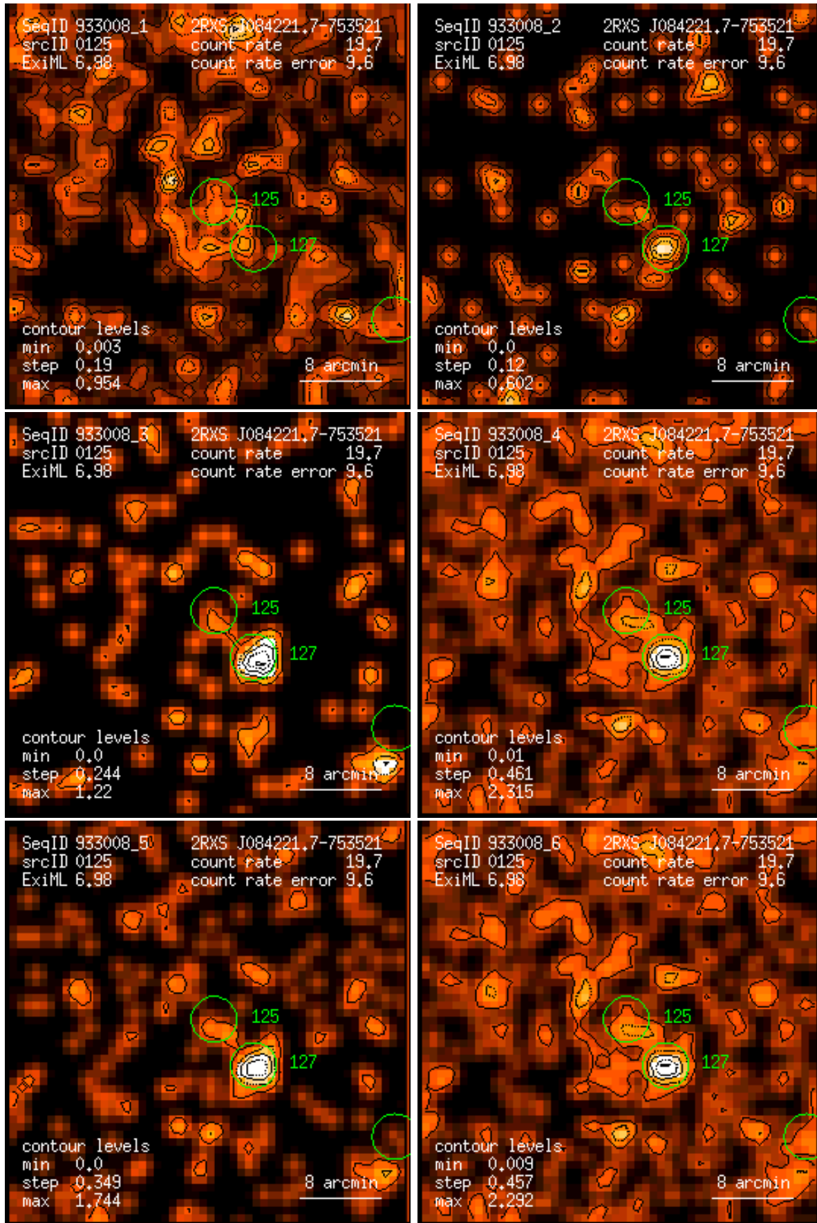
Figure 125: RASS 933008: detection 0125: band rate images, Gaussian filter: (1) PSPC channels 11 – 41, (2) 52 – 90, (3) 91 – 201, (4) 11 – 235, (5) 52 – 201, (6) 11 – 201. Broad band rates in counts/ks. Band rate contour levels in counts/ks/arcmin 2 .
