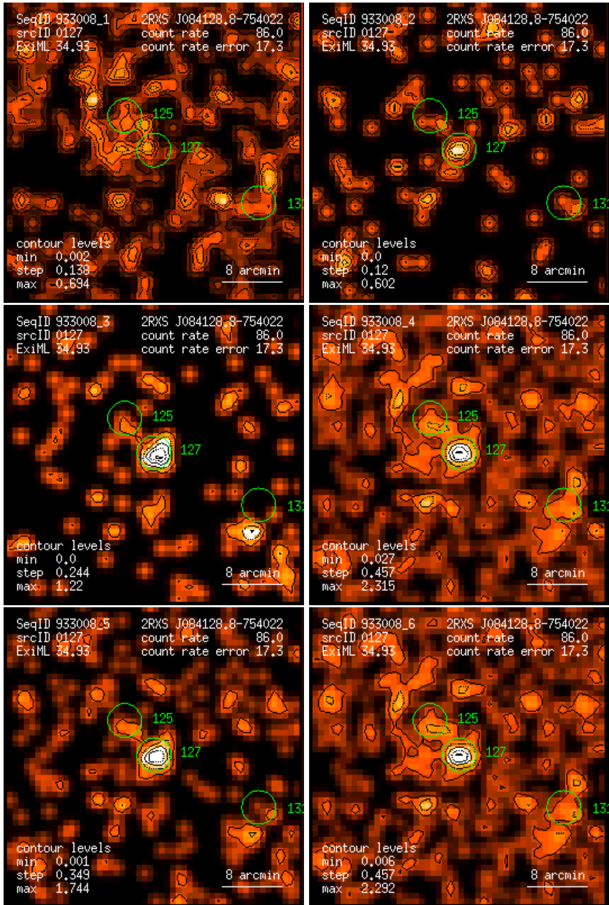
Figure 127: RASS 933008: detection 0127: band rate images, Gaussian filter: (1) PSPC channels 11 – 41, (2) 52 – 90, (3) 91 – 201, (4) 11 – 235, (5) 52 – 201, (6) 11 – 201. Broad band rates in counts/ks. Band rate contour levels in counts/ks/arcmin 2 .
