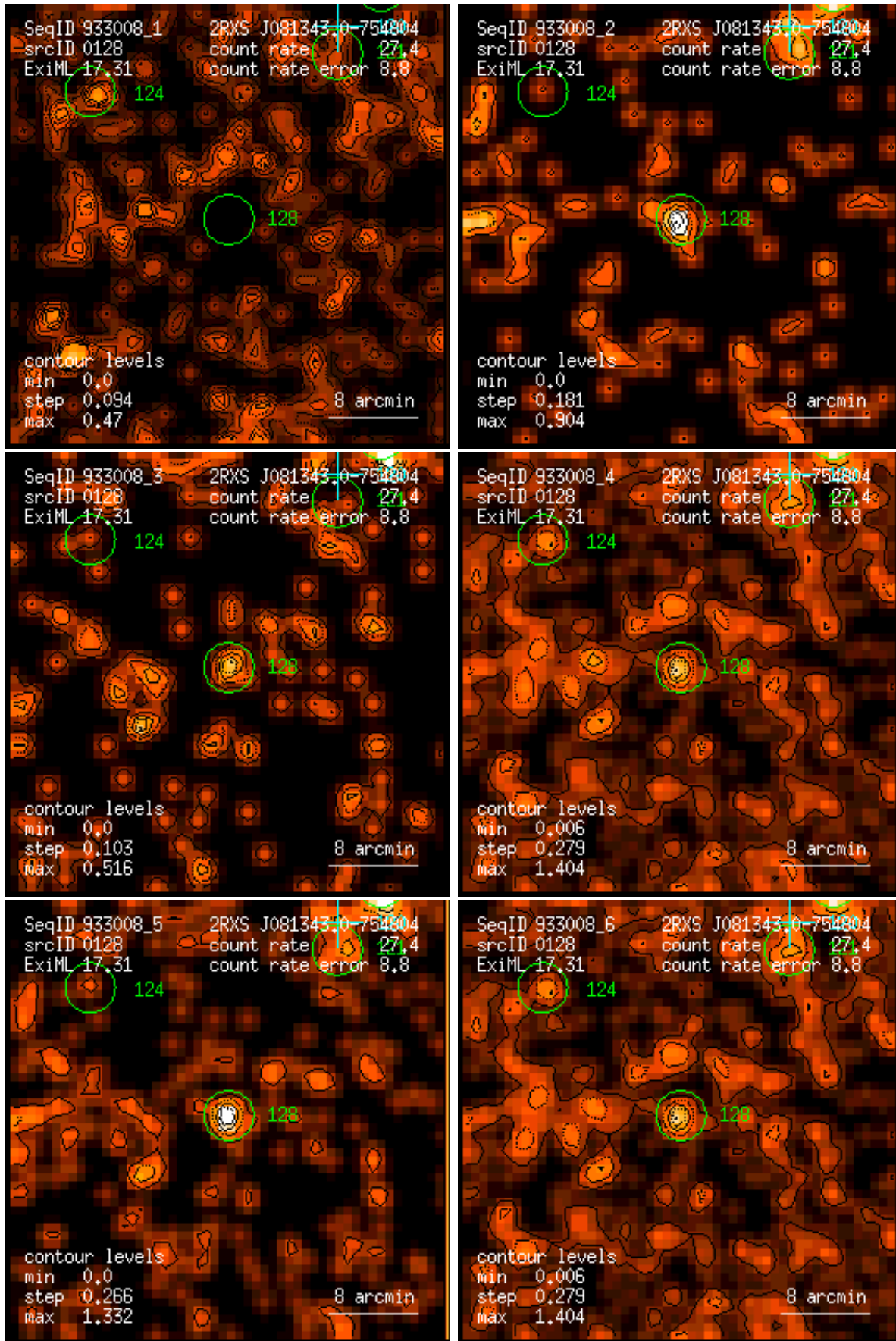
Figure 128: RASS 933008: detection 0128: band rate images, Gaussian filter: (1) PSPC channels 11 – 41, (2) 52 – 90, (3) 91 – 201, (4) 11 – 235, (5) 52 – 201, (6) 11 – 201. Broad band rates in counts/ks. Band rate contour levels in counts/ks/arcmin 2 .
