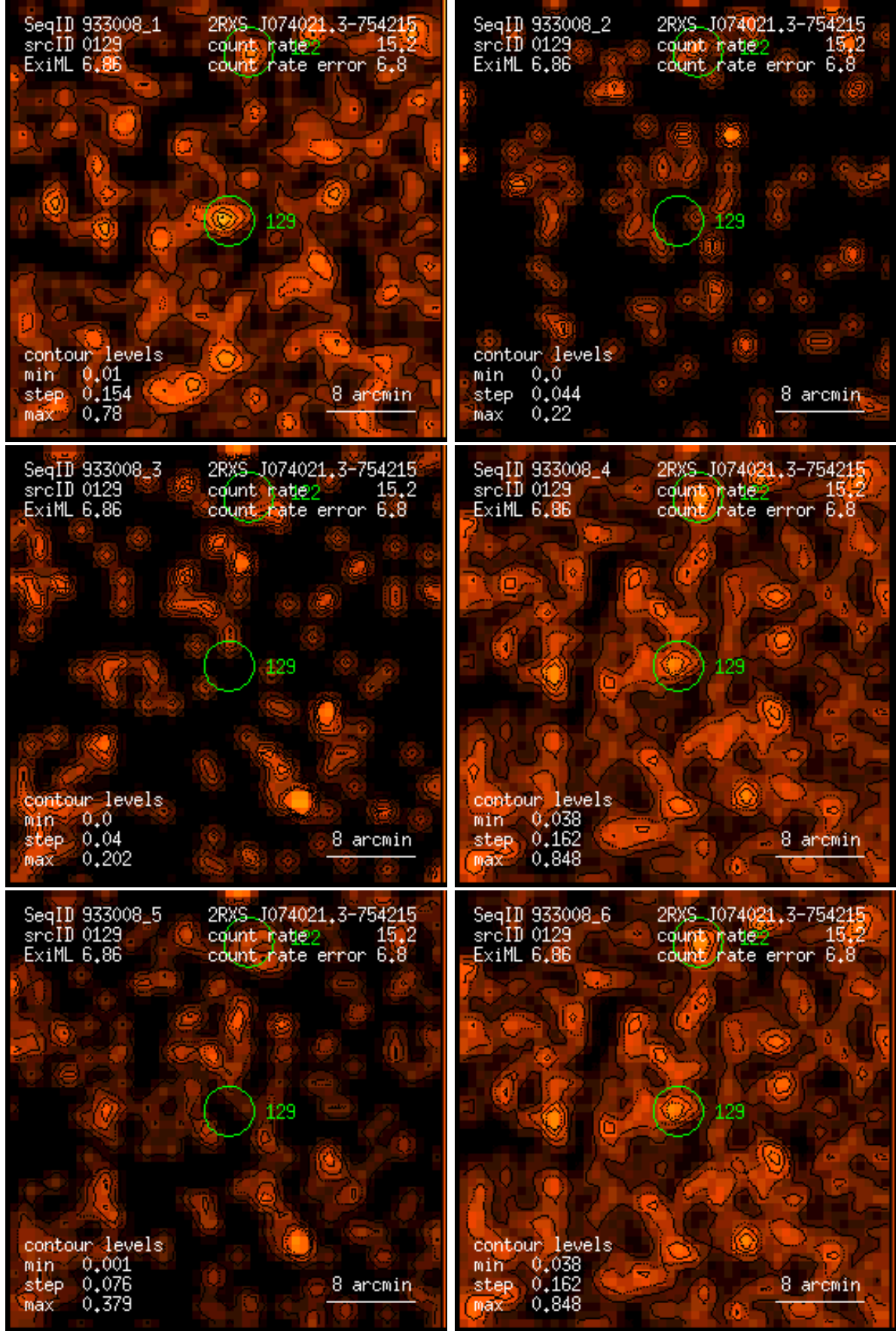
Figure 129: RASS 933008: detection 0129: band rate images, Gaussian filter: (1) PSPC channels 11 – 41, (2) 52 – 90, (3) 91 – 201, (4) 11 – 235, (5) 52 – 201, (6) 11 – 201. Broad band rates in counts/ks. Band rate contour levels in counts/ks/arcmin 2 .
