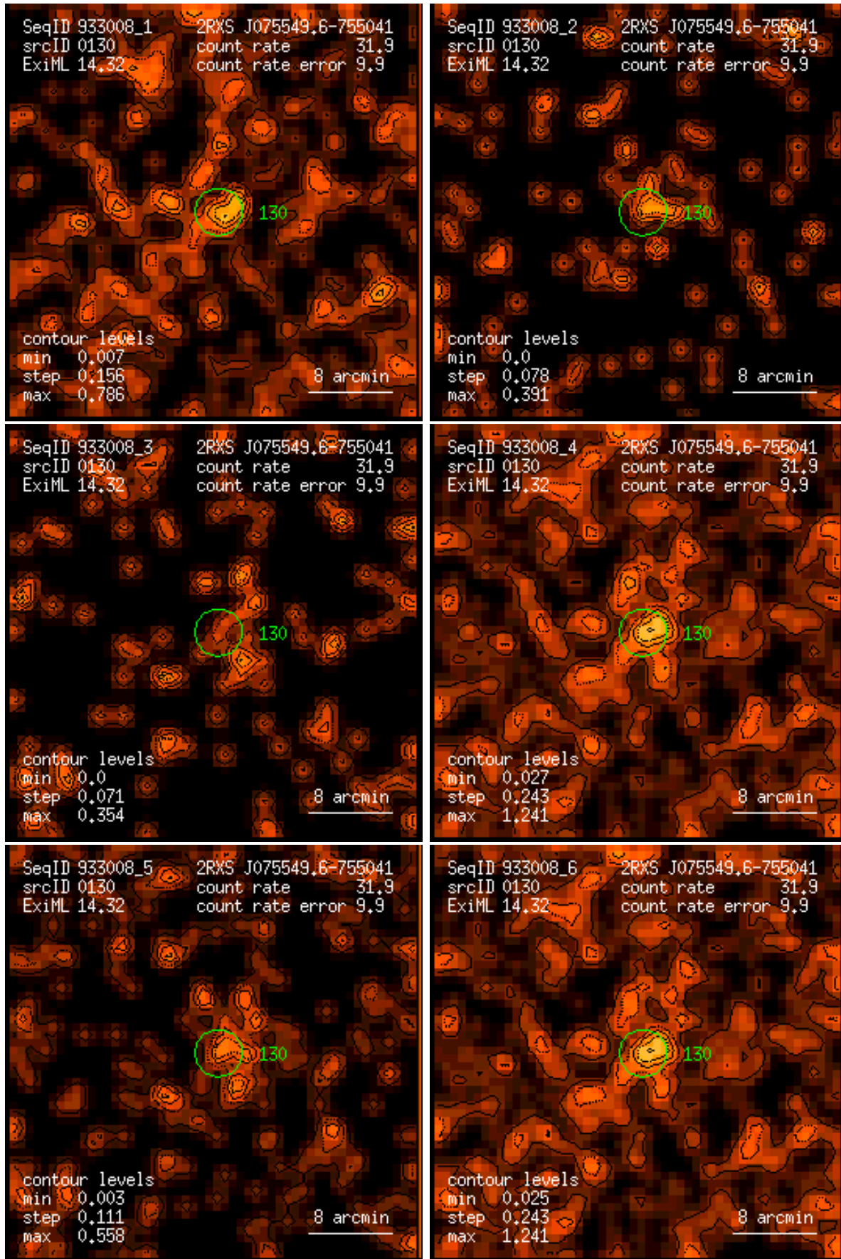
Figure 130: RASS 933008: detection 0130: band rate images, Gaussian filter: (1) PSPC channels 11 – 41, (2) 52 – 90, (3) 91 – 201, (4) 11 – 235, (5) 52 – 201, (6) 11 – 201. Broad band rates in counts/ks. Band rate contour levels in counts/ks/arcmin 2 .
