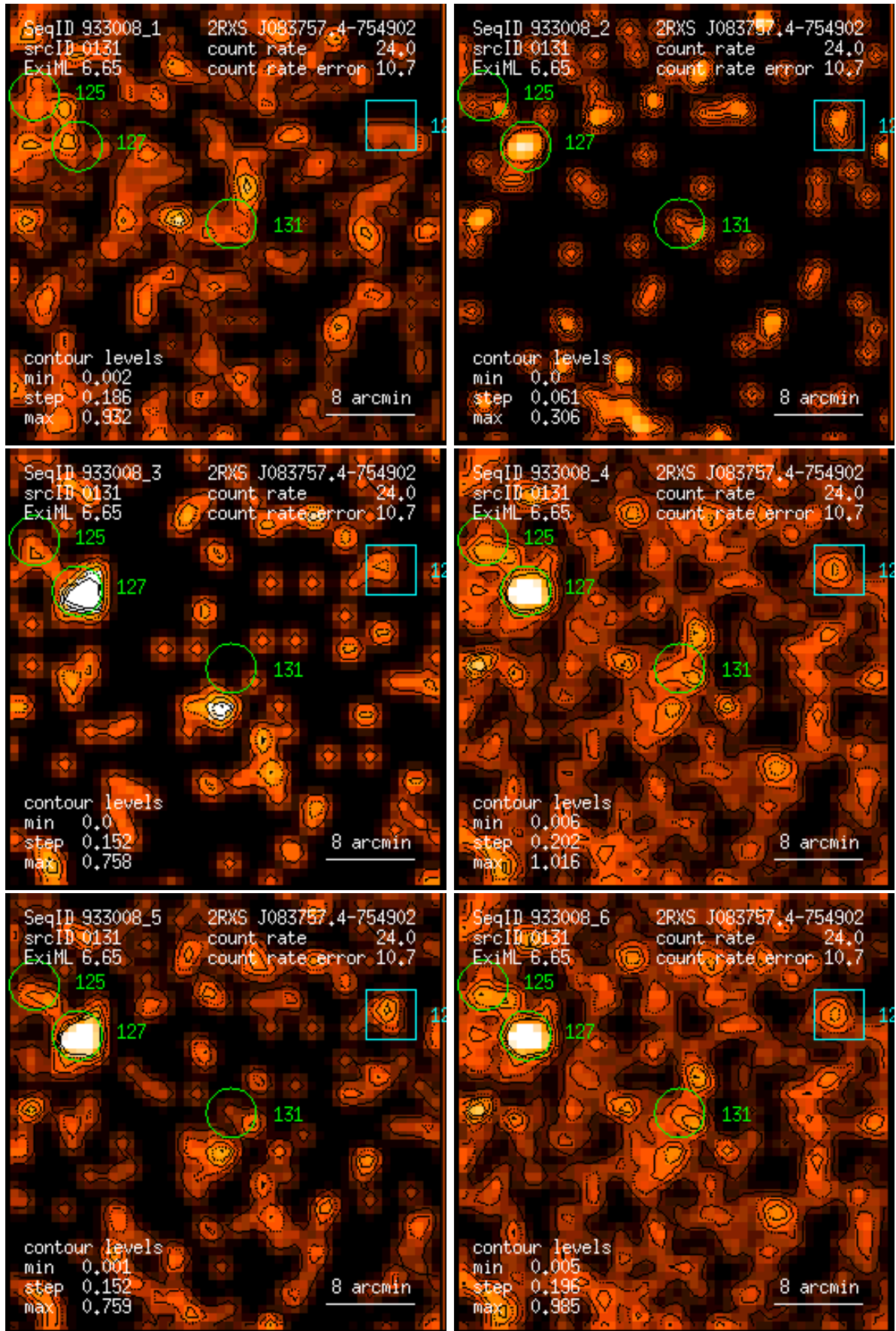
Figure 131: RASS 933008: detection 0131: band rate images, Gaussian filter: (1) PSPC channels 11 – 41, (2) 52 – 90, (3) 91 – 201, (4) 11 – 235, (5) 52 – 201, (6) 11 – 201. Broad band rates in counts/ks. Band rate contour levels in counts/ks/arcmin 2 .
