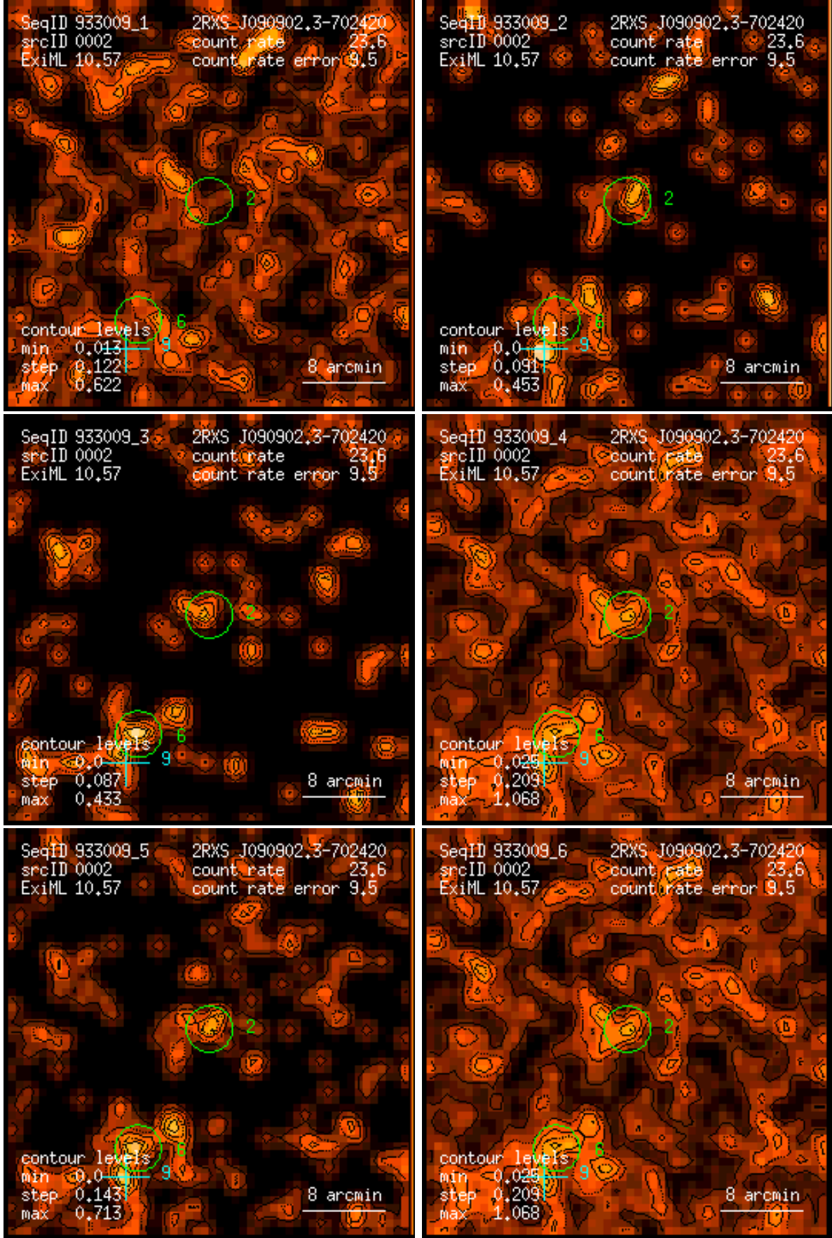
Figure 2: RASS 933009: detection 0002: band rate images, Gaussian filter: (1) PSPC channels 11 – 41, (2) 52 – 90, (3) 91 – 201, (4) 11 – 235, (5) 52 – 201, (6) 11 – 201. Broad band rates in counts/ks. Band rate contour levels in counts/ks/arcmin 2 .
