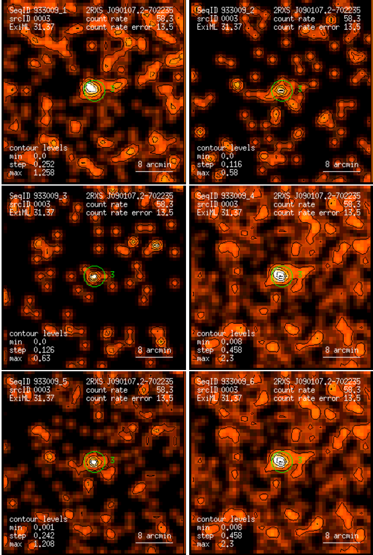
Figure 3: RASS 933009: detection 0003: band rate images, Gaussian filter: (1) PSPC channels 11 – 41, (2) 52 – 90, (3) 91 – 201, (4) 11 – 235, (5) 52 – 201, (6) 11 – 201. Broad band rates in counts/ks. Band rate contour levels in counts/ks/arcmin 2 .
