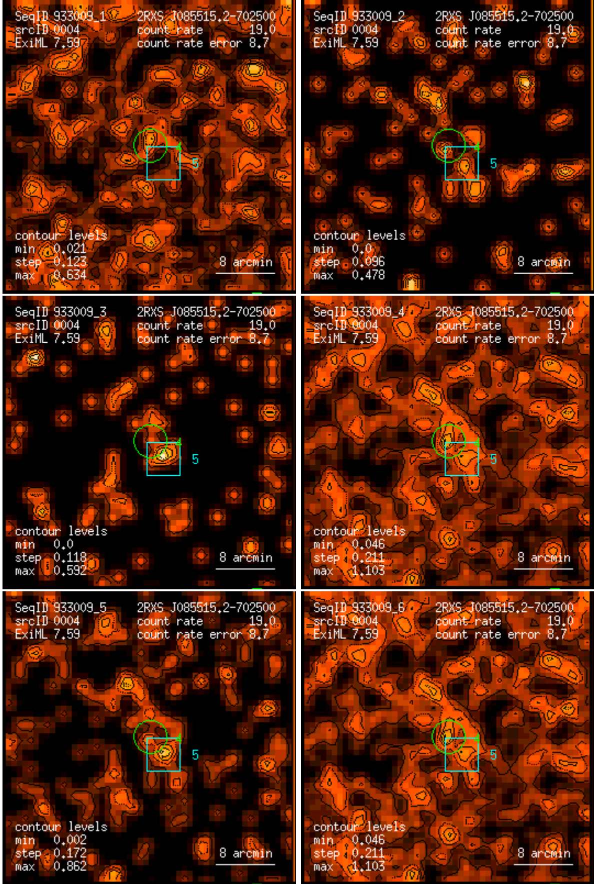
Figure 4: RASS 933009: detection 0004: band rate images, Gaussian filter: (1) PSPC channels 11 – 41, (2) 52 – 90, (3) 91 – 201, (4) 11 – 235, (5) 52 – 201, (6) 11 – 201. Broad band rates in counts/ks. Band rate contour levels in counts/ks/arcmin 2 .
