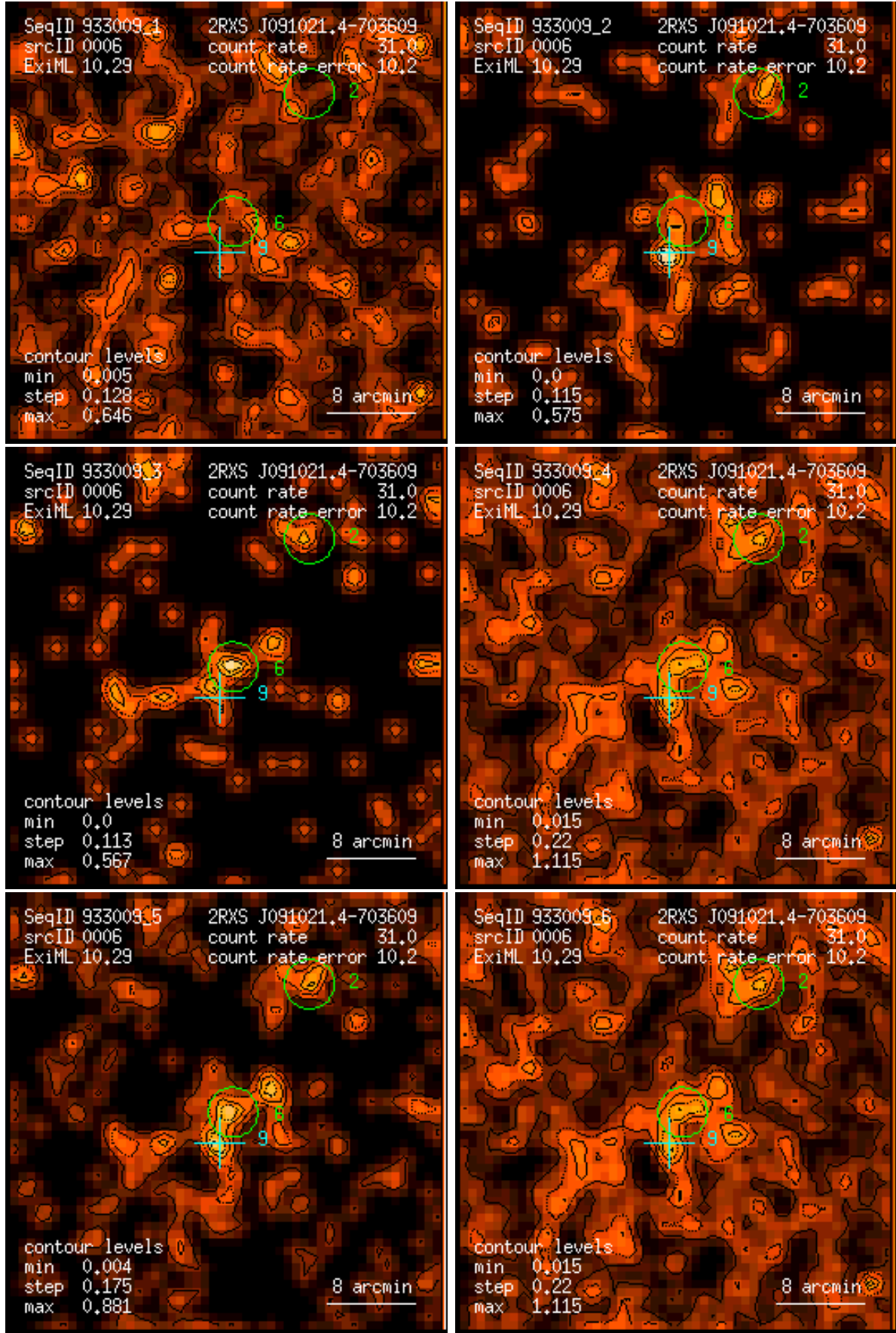
Figure 6: RASS 933009: detection 0006: band rate images, Gaussian filter: (1) PSPC channels 11 – 41, (2) 52 – 90, (3) 91 – 201, (4) 11 – 235, (5) 52 – 201, (6) 11 – 201. Broad band rates in counts/ks. Band rate contour levels in counts/ks/arcmin 2 .
