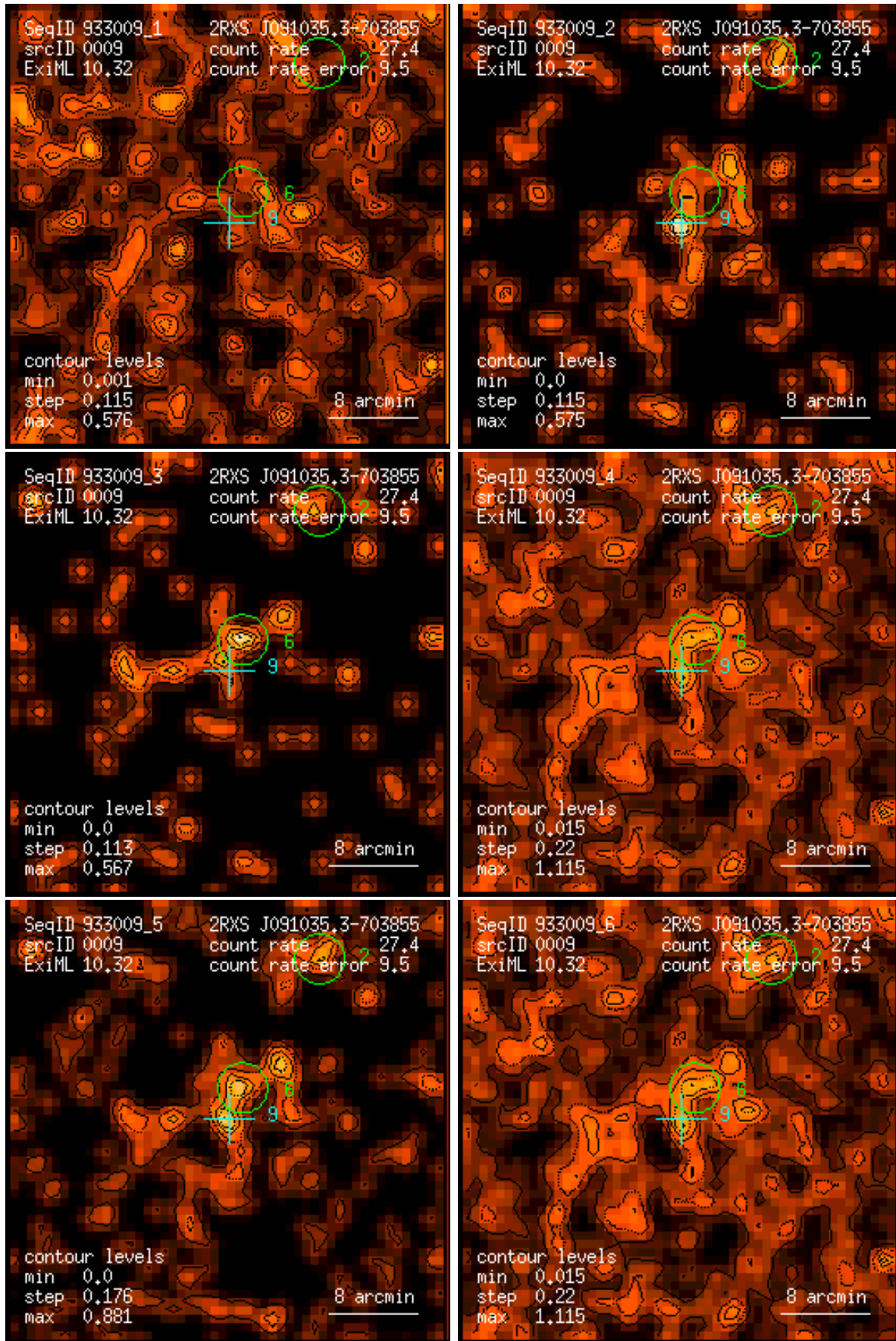
Figure 9: RASS 933009: detection 0009: band rate images, Gaussian filter: (1) PSPC channels 11 – 41, (2) 52 – 90, (3) 91 – 201, (4) 11 – 235, (5) 52 – 201, (6) 11 – 201. Broad band rates in counts/ks. Band rate contour levels in counts/ks/arcmin 2 .
