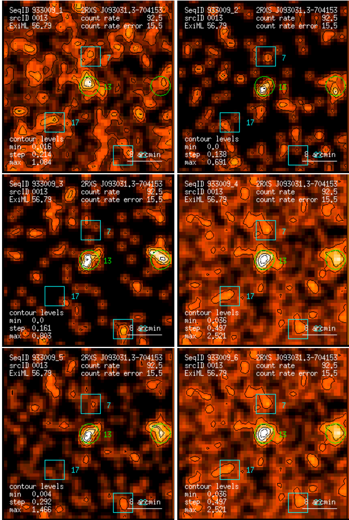
Figure 13: RASS 933009: detection 0013: band rate images, Gaussian filter: (1) PSPC channels 11 – 41, (2) 52 – 90, (3) 91 – 201, (4) 11 – 235, (5) 52 – 201, (6) 11 – 201. Broad band rates in counts/ks. Band rate contour levels in counts/ks/arcmin 2 .
